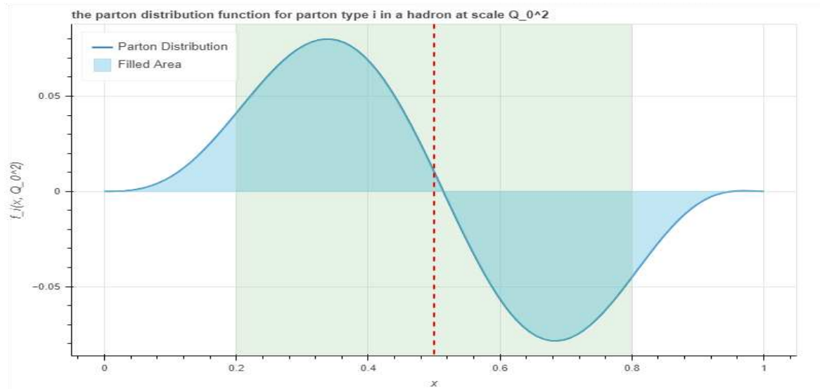
Figure 1. Parameterized Parton Distribution Functions.
