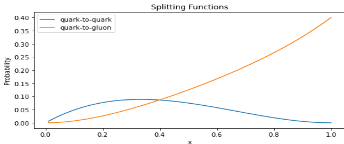
Figure 9. Splitting Functions ( P_{ij}(x) ), which delineate the probabilities of a quark splitting into another quark or a gluon.
