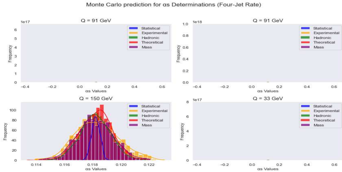
Figure 4. This figure presents Monte Carlo simulations for \alpha_s determinations associated with the Four-Jet Rate at various energy scales ( Q values). Each subplot corresponds to a specific Q value, showcasing the distribution of \alpha_s values considering different uncertainties: statistical (blue), experimental (orange), hadronic (green), theoretical (red), and mass-related (purple).
