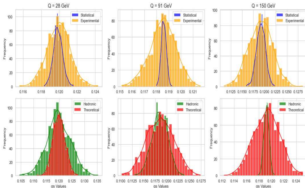
Figure 2. The plot illustrates Monte Carlo simulations for \alpha_s determinations at different energy scales (Q values). Each subplot corresponds to a specific Q value, showcasing the distribution of \alpha_s values considering various uncertainties: statistical (blue), experimental (orange), hadronic (green), and theoretical (red).
