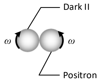
Figure 3. Schematic structure of a proton.
