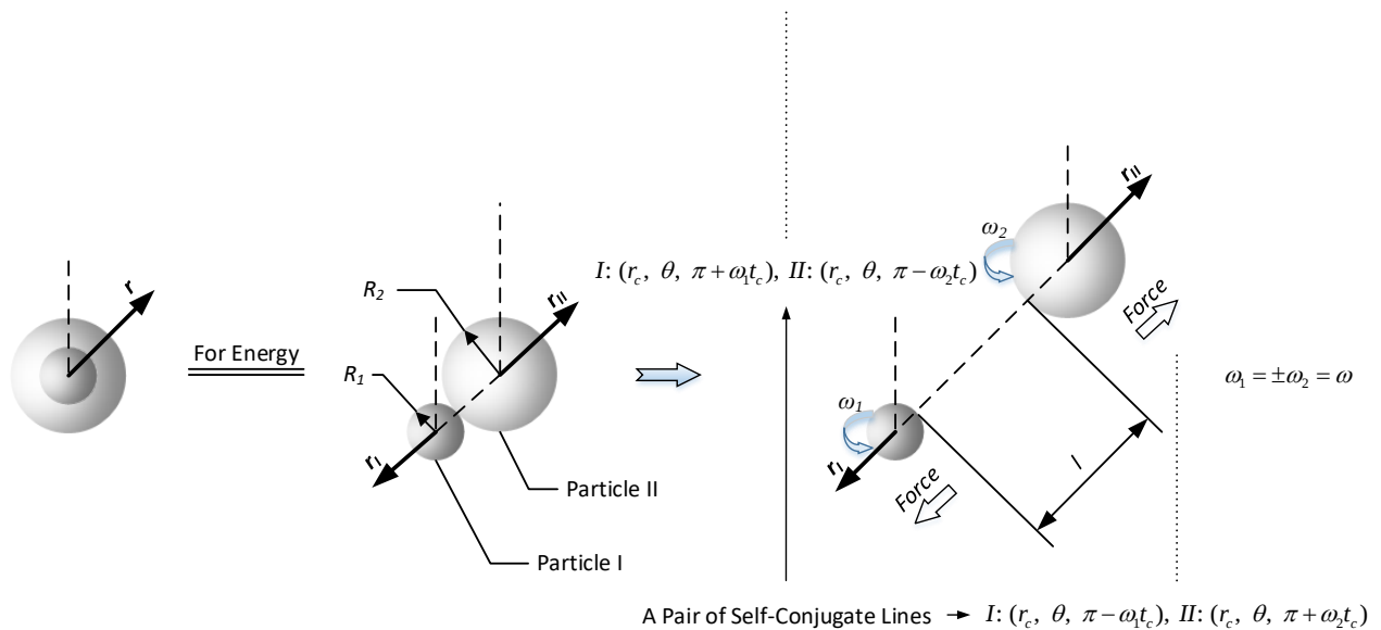
Figure 2. Energy conversion between two primary particles.
