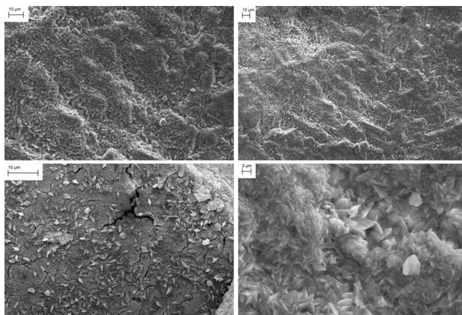
Figure 1. SEM images of weathered Carrara marble treated with a 5% w/w water solution of AmEtOxam-H 2 O.
