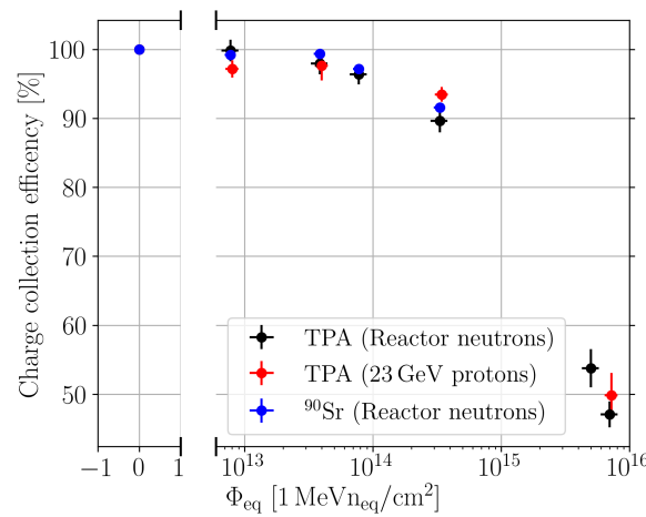
Figure 12. Charge collection efficiency for pad sensors, measured with the TPA-TCT and a ^{90}\text{Sr} setup, against the equivalent fluence. The type of irradiation is mentioned in the legend.
