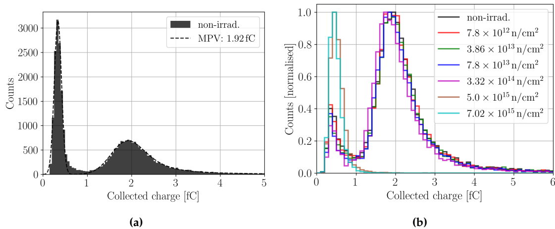
Figure 11. (a) Charge collection of a non-irradiated 156 \mu\text{m} thick p-type pad sensor measured in a ^{90}\text{Sr} setup. (b) Charge collection in neutron irradiated pad sensors for different fluences. The histogram is normalised to the maximum amount of counts to ease the comparison. The bias voltage in all measurements is 300 V.
