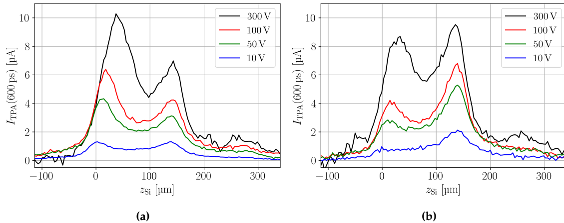
Figure 5. Prompt current at t_{pc} = 600 ps for different bias voltages measured for (a) a neutron fluence of 7.02 \times 10^{15} \text{ n/cm}^2 and (b) a proton fluence of 1.17 \times 10^{16} \text{ p/cm}^2 . The equivalent fluences are comparable. The double junction is clearly visible in both plots. The proton irradiated sample shows an electric field that grows from, and is stronger at, the back electrode. This effect is often called type inversion .
