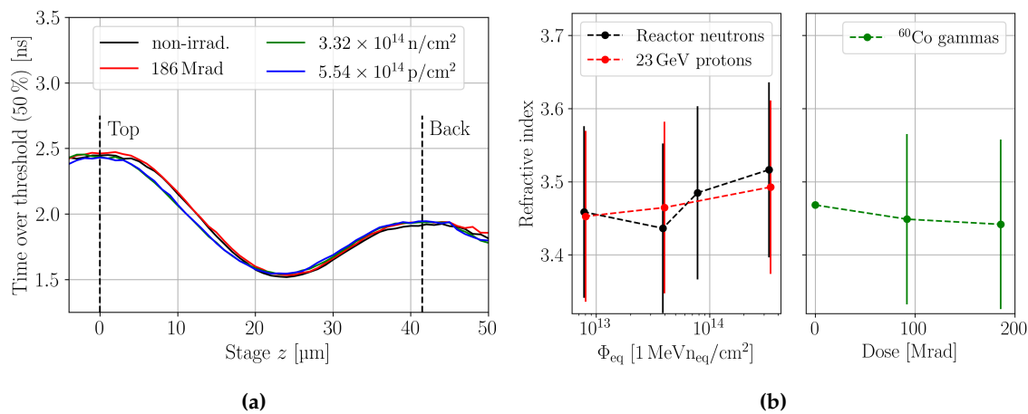
Figure 13. (a) Time over threshold profiles of the non-irradiated and the irradiated pad detectors. The highest fluences, while avoiding the double junction effect, are used to allow the comparison. The refraction from the air-silicon interface is not corrected in the z -axis. The location of the top and back interface is extracted from the non-irradiated device, and they are indicated by the dashed lines. (b) Refractive index extracted from the in-depth scans of various irradiated pad detectors. The nominal refractive index n(250 \text{ K}) = 3.4681(2) is taken from [30]. All scans are performed with a bias voltage of 300 V.
