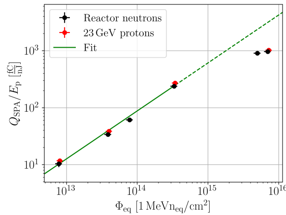
Figure 9. Charge collected by SPA normalised with the pulse energy for proton and neutron irradiated in 156 \mu\text{m} thick pad detectors, biased to 300 V. The fit function is of the form C \cdot \Phi_{\text{eq}}^a , with C = 14.3 \times 10^{-11} \text{ cm}^2 \text{a fC/nJ} and a = 0.84 . The highest fluences are excluded from the fit.
