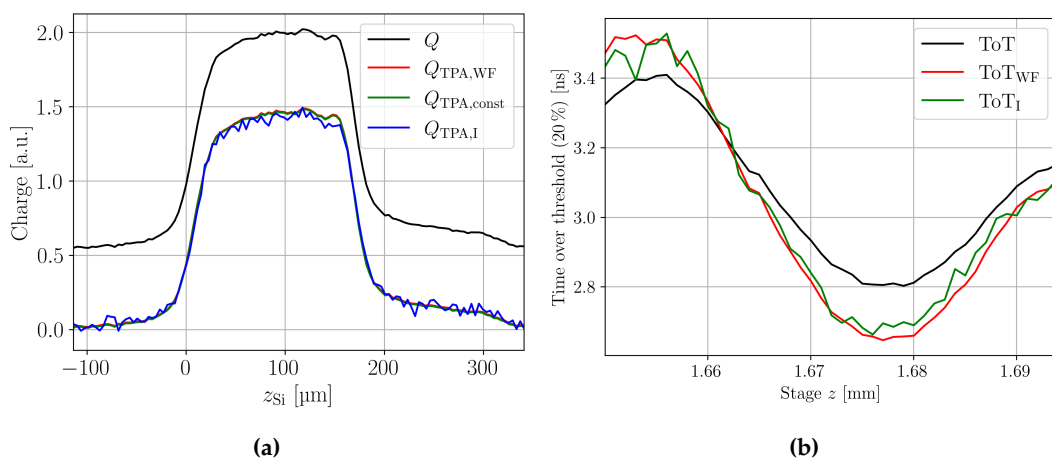
Figure 2. (a) Charge versus depth profile of an irradiated ( 3.32 \times 10^{14} n/cm) 156 \mu m thick p-type planar pad detector. The bias voltage is 300 V. A comparison of the three different SPA correction methods is shown. The waveform subtraction method is indicated by the index WF, the subtraction method by the index const , and the correction by intensity method by the index I. The uncorrected data are given without index. (b) Time over threshold measurement in the same pad detector, including a comparison of the waveform subtraction and the intensity correction method.
