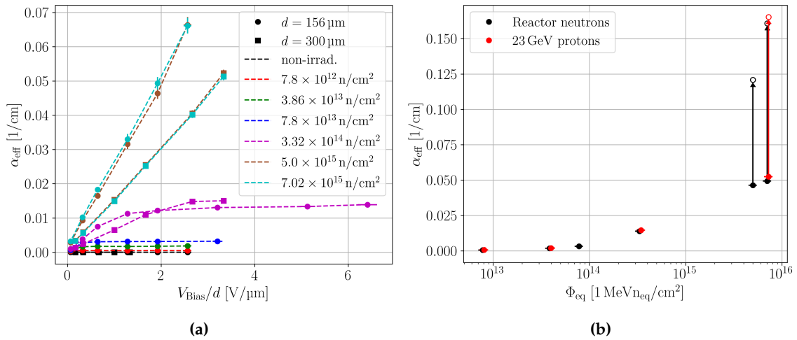
Figure 10. (a) Effective linear absorption coefficient of neutron irradiated pad detectors versus the bias voltage, which is normalised with the device thickness. (b) Effective linear absorption coefficient for 156 \mu\text{m} thick neutron and proton irradiated pad detectors versus the equivalent fluence. The value for the maximum bias voltage is used. The absorption coefficient does not saturate for the highest fluences and the highest applied bias voltage is different for the proton and neutron irradiated devices. In order to show comparable \alpha_{\text{eff}} for the highest fluences, a bias voltage of 300 V is selected. The arrows are used to guide the eye towards the empty markers. These show the \alpha_{\text{eff}} calculated from the interpolated Q_{\text{SPA}}(\Phi_{\text{eq}}) of Figure 9.
