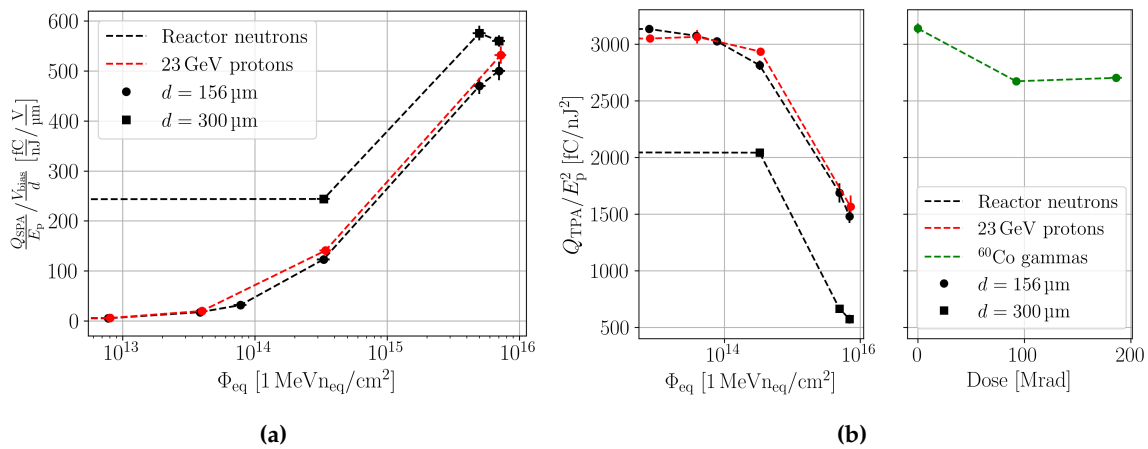
Figure 8. (a) SPA charge collection normalised with the average electric field versus the equivalent fluence for neutron and proton irradiated FZ p-type pad detector. (b) TPA charge collection versus the equivalent fluence and dose for the same DUT.
