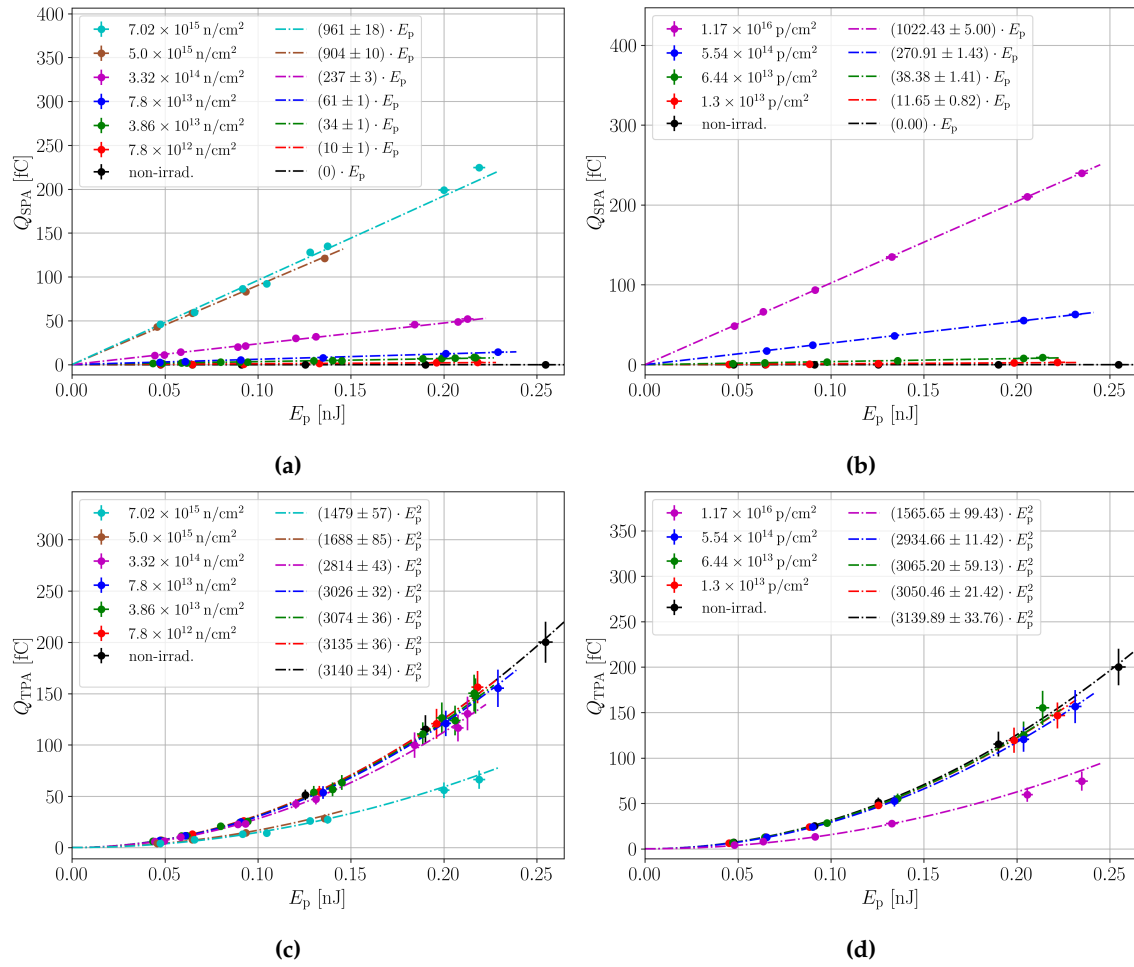
Figure 4. Charge collected by SPA in neutron (a) and proton (b) irradiated 156 \mu\text{m} thick pad sensors. Charge collected by TPA for the same neutron (c) and proton (d) irradiated devices. The TPA charge is extracted as the mean of the collected charge between the FWHM of the in-depth scans. The bias voltage for all scans is 300 V.
