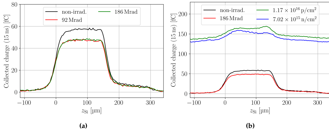
Figure 6. (a) In-depth scans of the charge collection in pad detectors. Gamma irradiated samples and a non-irradiated sample are shown. (b) Comparison between the in-depth scans of a non-irradiated, a neutron, a proton, and a gamma irradiated pad sensor. The bias voltage in all scans is 300 V.
