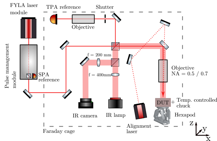
Figure 1. Sketch of the used table top TPA-TCT setup.
