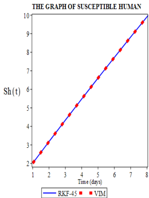
Fig 1 Solution comparison plot of the susceptible human population between variational iteration method and Runge-Kutta-Felhberg 45 (RKF-45).
