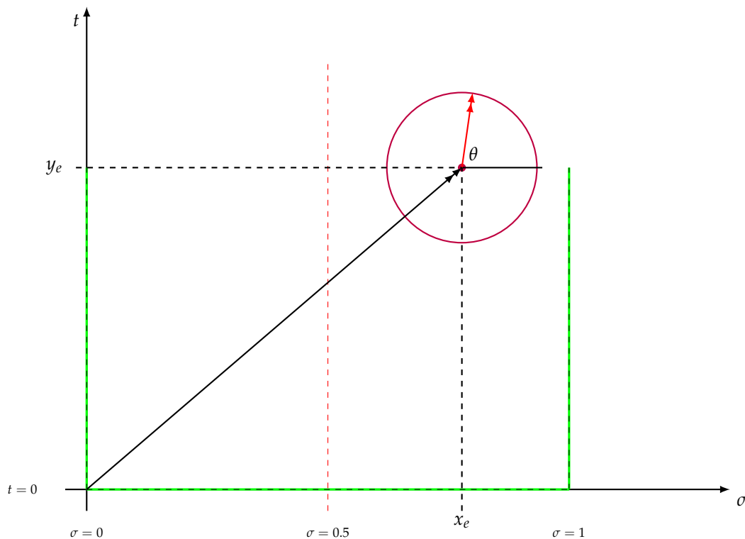
Figure 7. Relevant part of open critical strip and critical line
