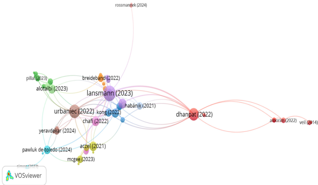
Figure 5. Bibliographic Coupling Network.
