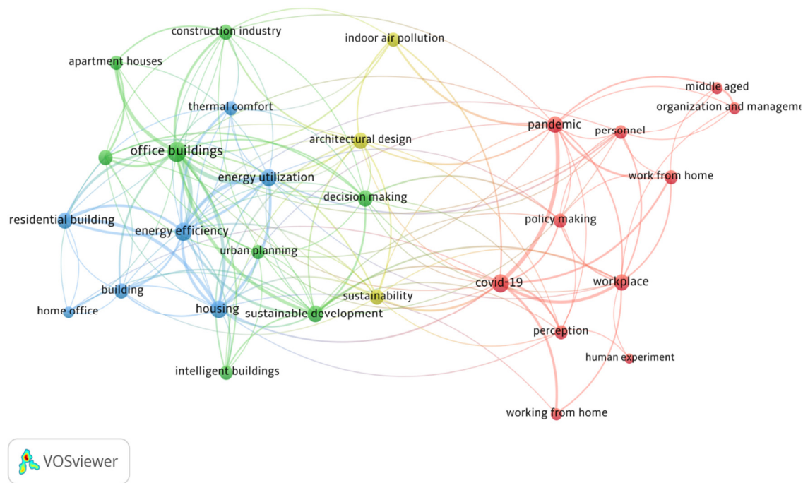
Figure 3. Co-Occurrence of Keywords in Clusters.
