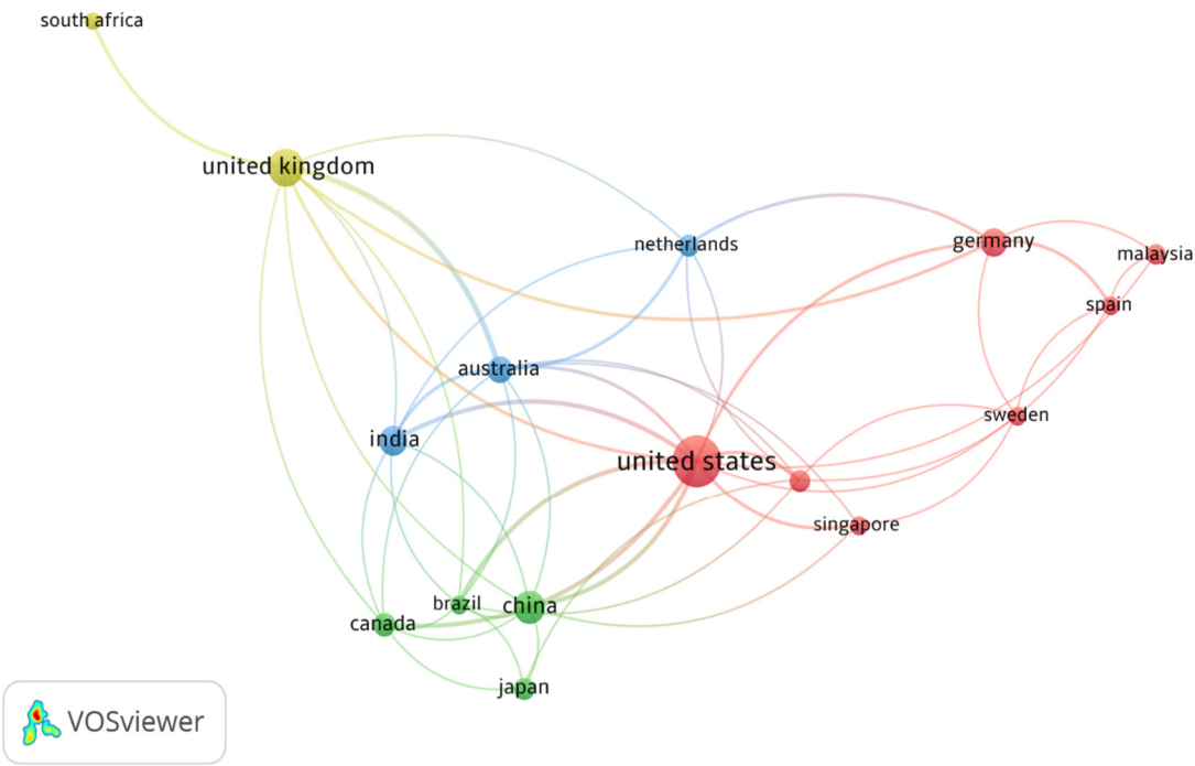
Figure 4. Network of Countries.
