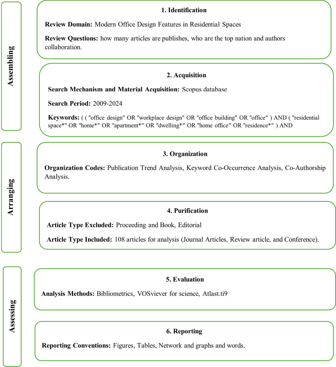
Figure 1. Overview of SPAR-4-SLR Protocol Framework.
