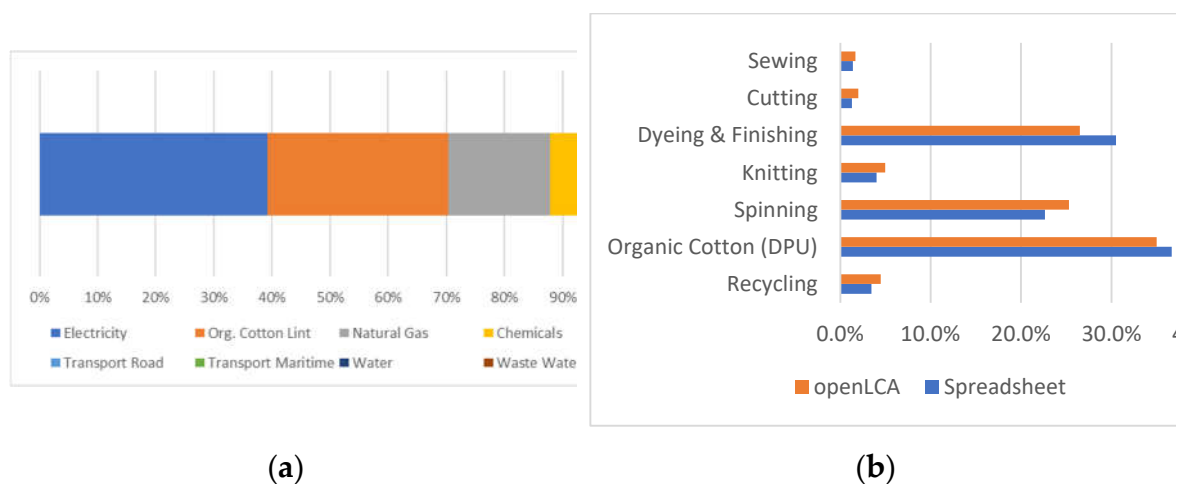
Figure 7. a) Percentage of GWP 100 impact per type per flow; (b) Percentage of GWP 100 impact per type per process and comparison of the spreadsheet and openLCA results. Organic Cotton (DPU) represents the impact generated by the organic lint cultivation, ginning and transportation from Turkey to recycling facility.
