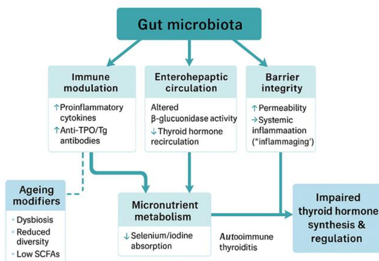
Figure 3. Proposed Mechanisms Linking Gut Microbiota and Thyroid Function in Ageing. (TPO/Tg antibodies=Thyroid peroxidase / thyroglobulin antibodies; SCF=short chain fatty acid).
