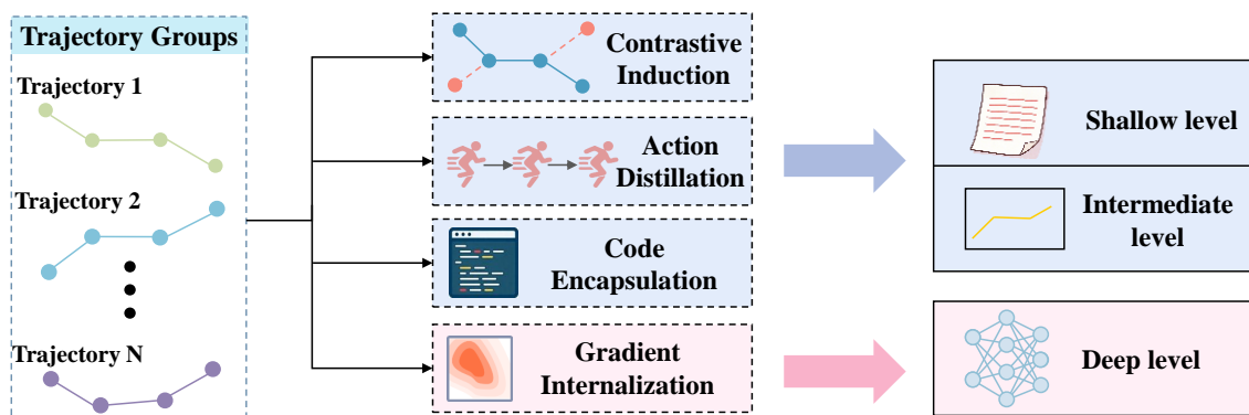
Figure 3. Overview of Cross-Trajectory Abstraction.
