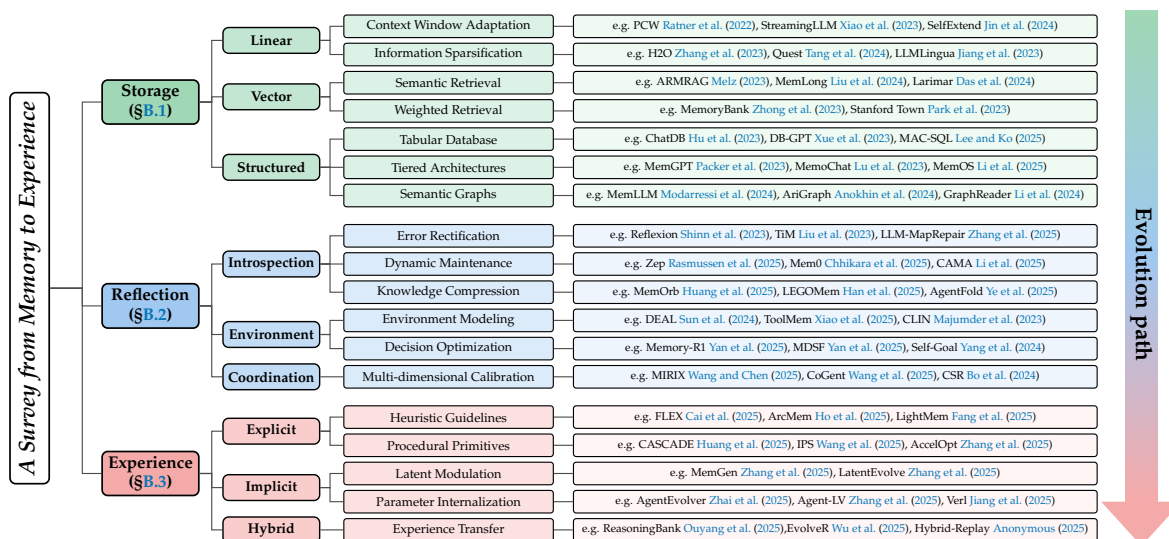
Figure 4. Taxonomy of LLM agent Memory Mechanisms
