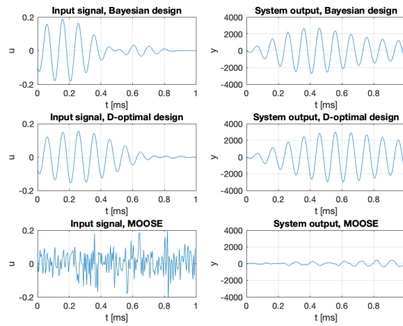
Figure 3. Optimal input signals (left) and corresponding system outputs (right) obtained by maximizing the Bayesian criterion (??) (top), the averaged D-optimal criterion (104) (middle), and the spectral criterion (87), subject to the constraint (3) with \tilde{\mathbf{U}} = 0 . Maximization of the spectral criterion (87) was performed using the MOOSE-2 solver evaluated at \theta = m_\theta = 55 . The norm of all signals is equal to 1, and the scale is consistent across all plots.
