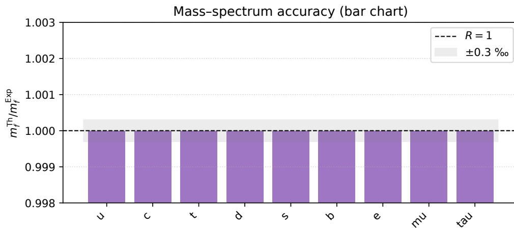
Figure A13. Mass-ratio bar chart: grey band = \pm 0.3\% , dashed line = exact match.
