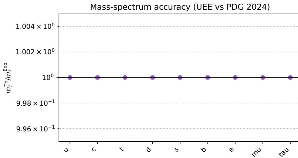
Figure A6. Mass ratios m_f^{Th}/m_f^{Exp} (logarithmic).
