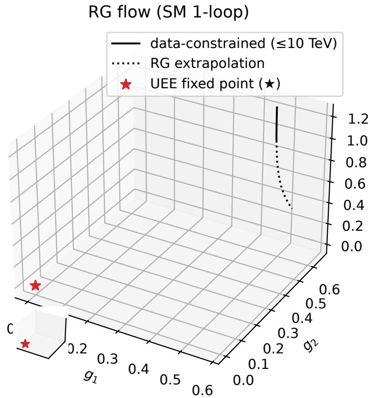
Figure A9. RG flow (3D). Thick solid line = measured region, dotted = extrapolation. ★ = UEE fixed point.
