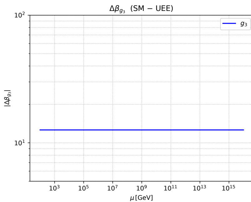
Figure A4. Plot of \Delta\beta_{g_3} only.
