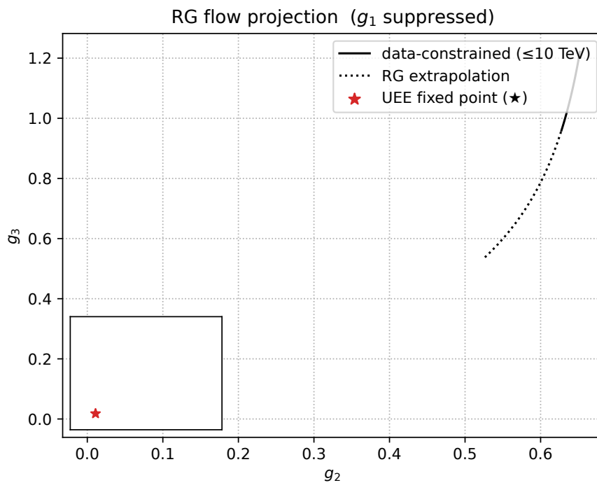
Figure A10. Projection onto the g_2 - g_3 plane. Symbols are the same as in Fig. A9.
