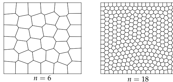
Figure 8. Meshes with 6 \times 6 and 18 \times 18 elements.
