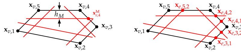
Figure 6. The two sub-partitions of E_5 used for constructing specific H^p supplemental functions. The left one is used for \mathcal{DS}_r^M and \mathbf{V}_r^{M,s} , where h_M = \lambda_5(\mathbf{x}_{e,4}^M) . The right one is used for \mathcal{DS}_r^T and \mathbf{V}_r^{T,s} , where the closest trisection points are marked in red.
