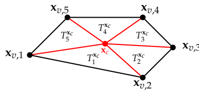
Figure 4. Sub-triangulation based on a center point. Shown is \mathcal{T}^{x_c}(E_5) using the centroid x_c .
