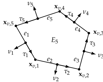
Figure 1. A pentagon E_5 , with edges e_i , outer unit normals \nu_i , tangents \tau_i , and vertices \mathbf{x}_{v,i} .
