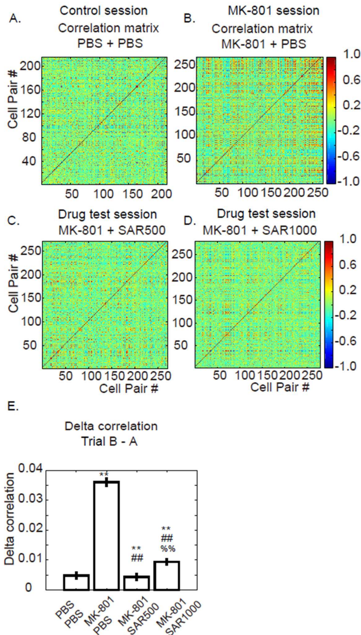
Figure 3. Examples of dorsal CA1 cell-cell correlation matrixes from Mouse #3. (A) to (D) Cell-cell correlation matrixes after the administration of PBS + PBS, MK-801 + PBS, MK-801 + SAR500, and MK-801 + SAR1000, respectively. (E) Delta correlation coefficient (trial B – trial A) of pairwise neurons of all animals (Mean ± SEM) (Each single cell was treated as a sample for bootstrapping before statistical analysis). **: vs. PBS + PBS; ##: vs. MK-801 + PBS; %: vs. MK-801 + SAR500 indicates significant difference ( p < 0.01 ), as determined using the Bootstrap method followed by Tukey's post hoc test for multiple comparisons.
