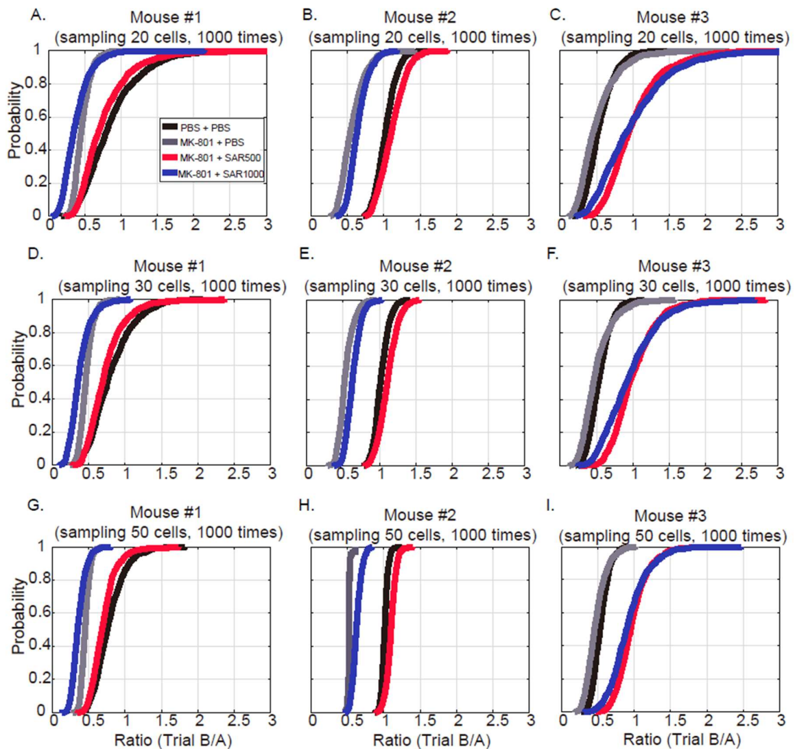
Figure 2. Fluorescence intensity ratio of trial B/trial A of grouped cell ensembles. (A) to (C) Cumulative distribution of the intensity ratio which are randomly sampled and averaged 20 intensity traces 1000 times in mouse #1 to #3, respectively. The manipulations of PBS + PBS, MK-801 + PBS, MK-801 + SAR500, and MK-801 + SAR1000 are represented by black, gray, red, and blue lines. (D) to (F) Intensity ratio which are randomly selected and averaged 30 intensity traces 1000 times. (G) to (I) Intensity ratio which are randomly selected and averaged 50 intensity traces 1000 times.
