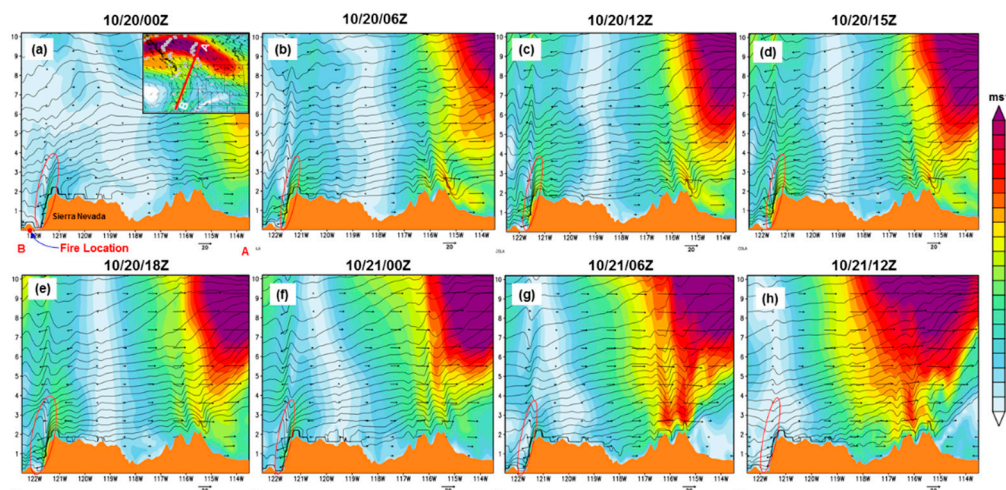
Figure 12. Cross-section along AB (denoted in the upper-right corner) from the WRF (d01) simulation of isotachs (shaded; ms -1 ), isentropes (contour lines; K), and wind barbs. The cross-section line passes through the jet streak's right exit region and the fire location at 250 hPa level.
