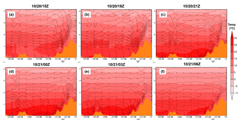
Figure A2. Vertical cross-section from the WRF (d03) simulation of temperature (shaded; °C), isentropes (contour lines; K), and wind barbs from 10/20/15Z to 10/21/06Z. The cross-section is along line CD (denoted in Figure 14).
