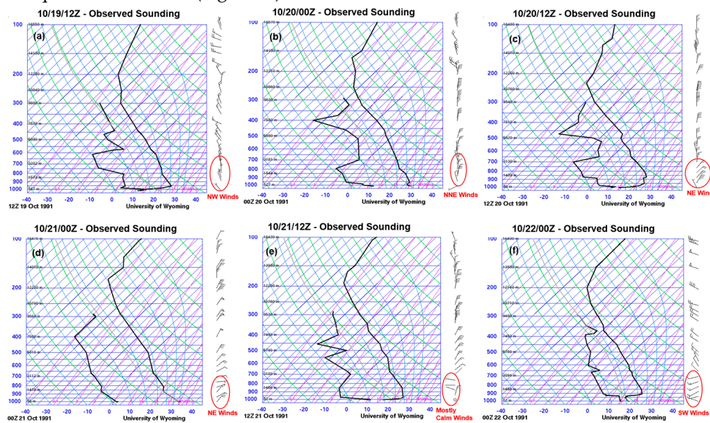
Figure 4. Observed thermodynamic diagram for Oakland International Airport valid at (a) 1200 UTC Oct 19, (b) 0000 UTC Oct 20, (c) 1200 UTC Oct 20, (d) 0000 UTC Oct 21 and (e) 1200 UTC Oct 21 and (f) 0000 UTC Oct 22. The solid line on the left denotes dewpoint temperature, and on the right is temperature.
