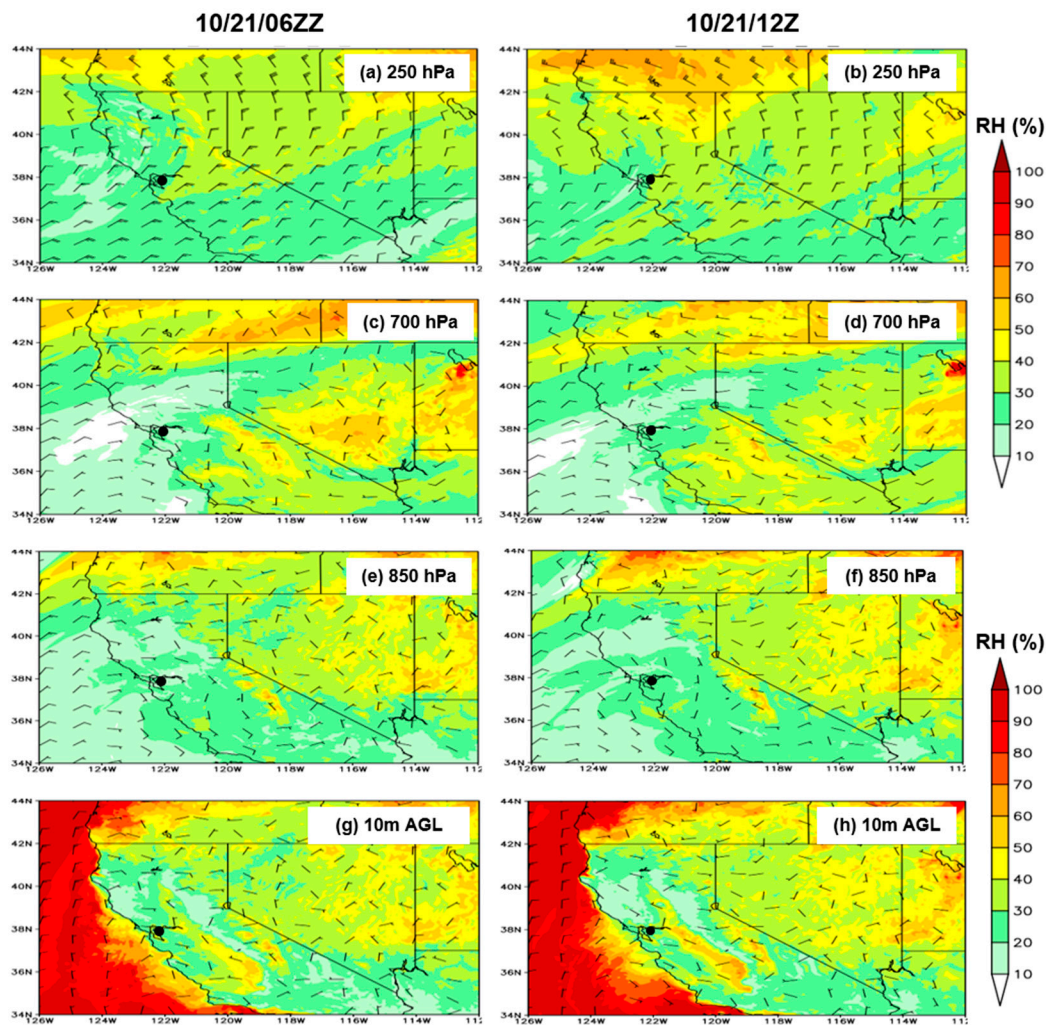
Figure 8. WRF (d02) simulation of RH (shaded; %) and wind barbs of (a),(b) 250 hPa, (c),(d) 700 hPa, (e),(f) 850 hPa, and (g),(h) 10m above ground level at (left) 0600 UTC Oct 21 and (right) 1200 UTC Oct 21.
