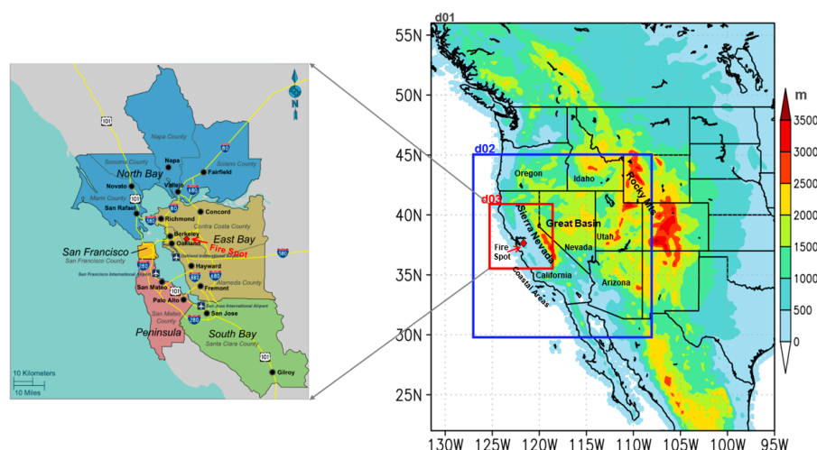
Figure 1. Domain set up for the East Bay Hills Fire (1991) with three nested domains with grid resolutions of 16km (d01), 4km (d02), and 1km (d03). On the left-hand side is the zoomed-in of the San Francisco Bay area and the East Bay Hills Fire location.
