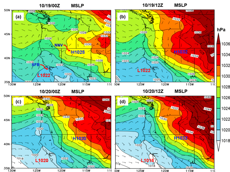
Figure 3. North American Regional Reanalysis (NARR) data of MSLP (shaded and contour lines; hPa) and wind barbs at (a) 10/19/00Z, (b) 10/19/12Z, (c) 10/20/00Z, and (d) 10/20/12Z. NNV indicates northern Nevada, and SFB is San Francisco Bay.
