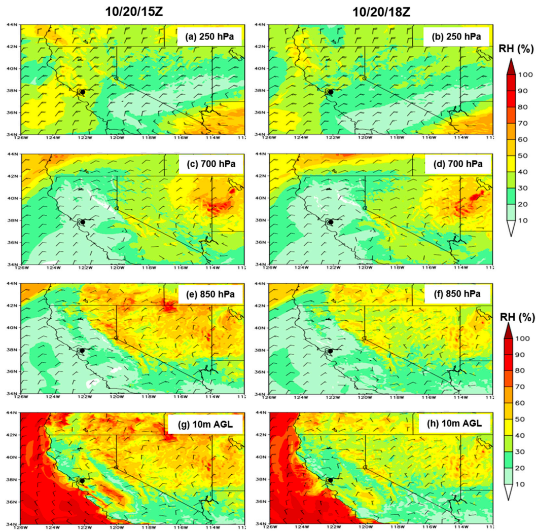
Figure 7. WRF (d02) simulation of RH (shaded; %) and wind barbs of (a),(b) 250 hPa, (c),(d) 700 hPa, (e),(f) 850 hPa, and (g),(h) 10m above ground level at (left) 1500 UTC Oct 20 and (right) 1800 UTC Oct 20.
