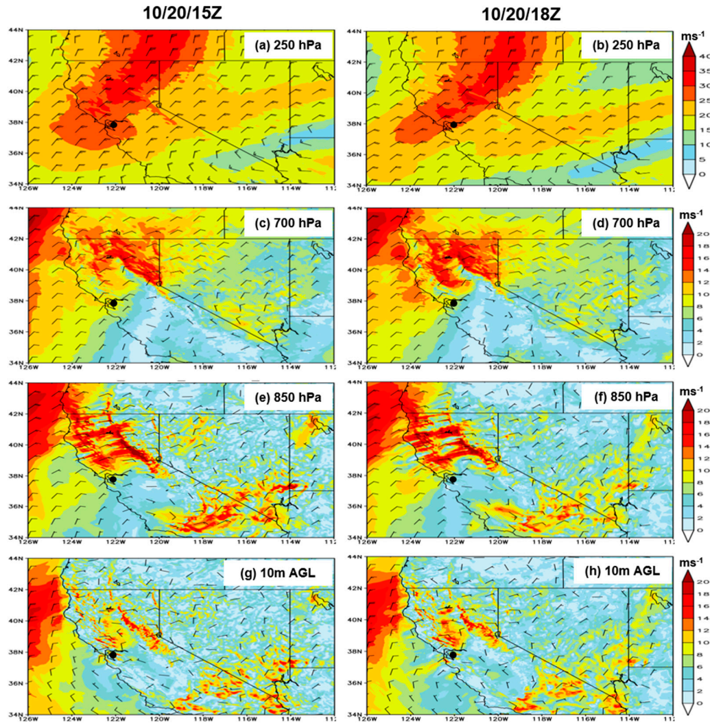
Figure 5. WRF (d02) simulation of isotachs (shaded; \text{ms}^{-1} ) and wind barbs at (a),(b) 250 hPa, (c),(d) 700 hPa, (e),(f) 850 hPa and (g),(h) 10m above ground level at (left) 1500 UTC Oct 20 and (right) 1800 UTC Oct 20.
