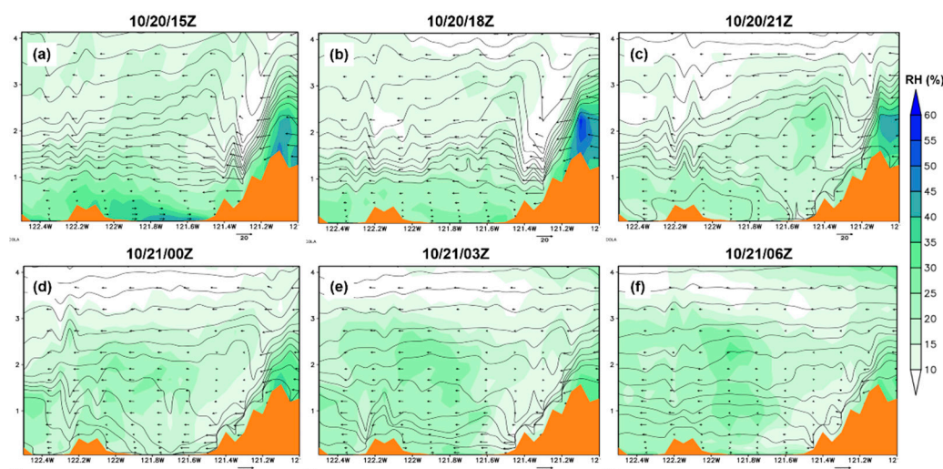
Figure A3. Vertical cross-section from the WRF (d03) simulation of RH (shaded; %), isentropes (contour lines; K), and wind barbs from 10/20/15Z to 10/21/06Z. The cross-section is along line CD (denoted in Figure 14).
