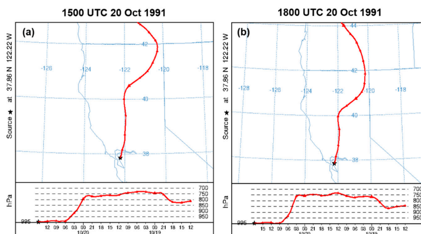
Figure 11. Backward trajectory analysis of winds from the NARR meteorological data starting from the fire location (37.86°N, 122.22°W) starting at 1500 UTC Oct 20, 1991 (a) and 1800 UTC October 20, 1991 (b). They all end at 1200 UTC Oct 18, 1991.
