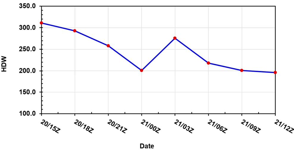
Figure 18. Time series of the HDW using WRF (d02) simulated data at the fire location (37.86° N latitude and 122.22° W longitude) from 10/20/15Z to 10/21/12Z.
