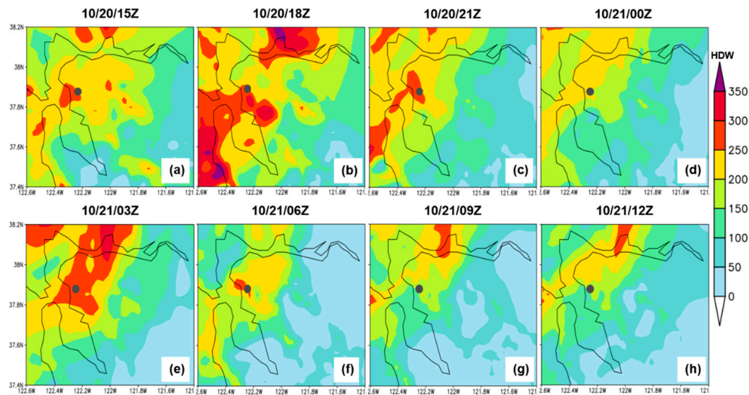
Figure 17. Maximum HDW (shaded) using WRF (d02) simulated data from 10/20/15Z to 10/21/12Z. The black dot indicates the fire location (37.86° N latitude and 122.22° W longitude).
