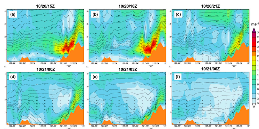
Figure A1. Vertical cross-section from the WRF (d03) simulation of Isotachs (shaded; ms-1), isentropes (contour lines; K), and wind barbs from 10/20/15Z to 10/21/06Z. The cross-section is along line CD (denoted in Figure 14).
