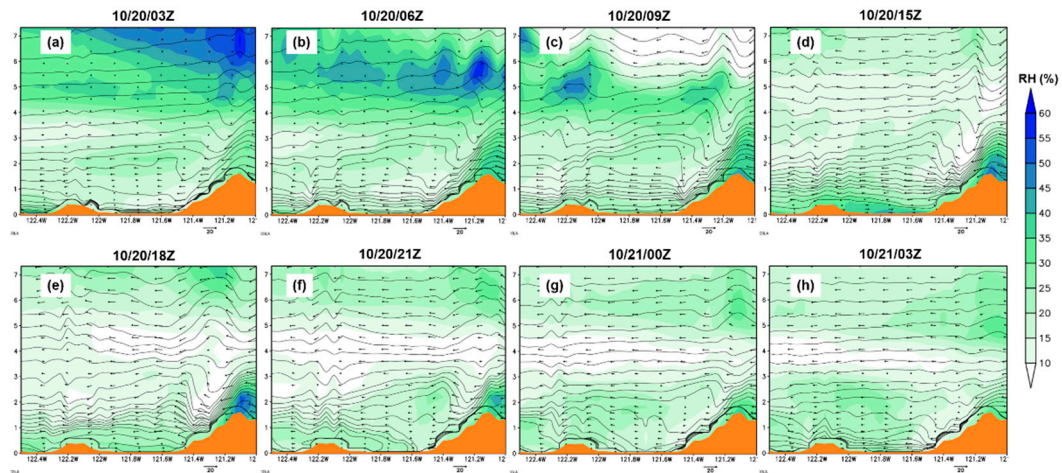
Figure 16. Cross-section along line CD (denoted in Figure 14) from the WRF (d02) simulation of RH (shaded; %), isentropes (contour lines; K), and wind barbs from 10/20/03Z to 10/21/03Z.
