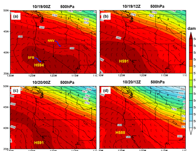
Figure 2. North American Regional Reanalysis (NARR) data of 500 hPa geopotential height (shaded) and wind barbs valid at (a) 10/19/00Z, (b) 10/19/12Z, (c) 10/20/00Z, and (d) 10/20/12Z. NNV indicates northern Nevada, and SFB is San Francisco Bay.
