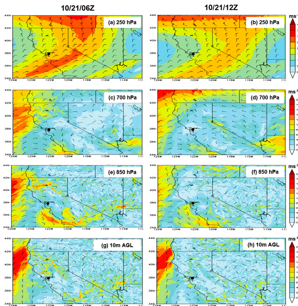
Figure 6. WRF (d02) simulation of isotachs (shaded; \text{ms}^{-1} ) and wind barbs of (a),(b) 250 hPa, (c),(d) 700 hPa, (e),(f) 850 hPa and (g),(h) 10m above ground level at (left) 0600 UTC Oct 21 and (right) 1200 UTC Oct 21.
