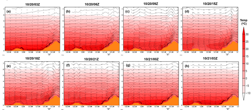
Figure 15. Cross-section along line CD (denoted in Figure 14) from the WRF (d02) simulation of temperature (shaded; °C), isentropes (contour lines; K), and wind barbs from 10/20/03Z to 10/21/03Z.
