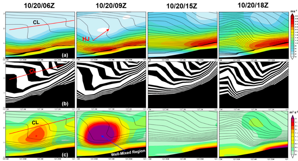
Figure 13. Vertical cross-section at the lee side of Sierra Nevada using the WRF (d02) simulation of (a) isotachs (shaded; \text{ms}^{-1} ) and isentropes (contour lines; K), (b) isentropes (shaded; K), and (c) TKE (shaded; \text{m}^2\text{s}^{-2} ) and isentropes (contour lines; K) from 10/20/06Z to 10/20/18Z. CL represents a critical level, and HJ means hydraulic jump.
