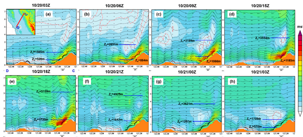
Figure 14. Cross-section along line CD (indicated in the upper-left panel) from the WRF (d02) simulation of isotachs (shaded; ms -1 ), isentropes (contour lines; K), and wind barbs. The red dashed lines represent the level where wind reversal occurs. The two horizontal lines are critical level heights calculated using Clark and Peltier's resonant amplification (upper) and Smith's hydraulic mechanisms (upper & lower).
