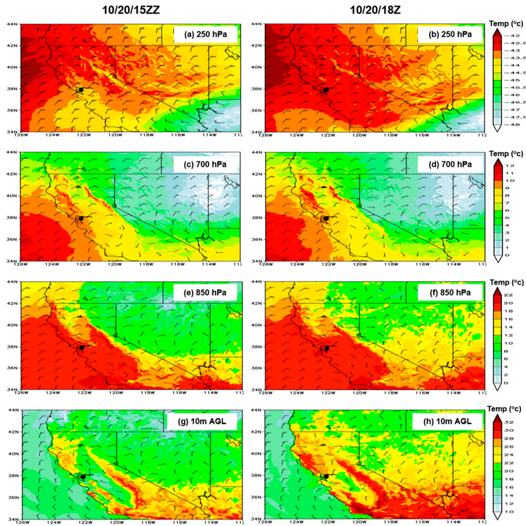
Figure 9. WRF (d02) simulation of temperature (shaded; °C) and wind barbs of (a),(b) 250 hPa, (c),(d) 700 hPa, (e),(f) 850 hPa, and (g),(h) 10m above ground level at (left) 1500 UTC Oct 20 and (right) 1800 UTC Oct 20.
