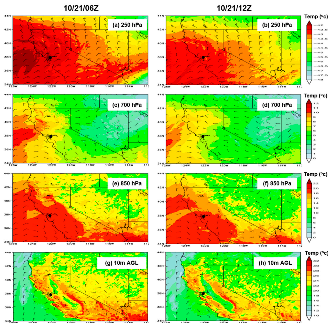
Figure 10. WRF (d02) simulation of temperature (shaded; °C) and wind barbs of (a),(b) 250 hPa, (c),(d) 700 hPa, (e),(f) 850 hPa, and (g),(h) 10m above ground level at (left) 0600 UTC Oct 21 and (right) 1200 UTC Oct 21.
