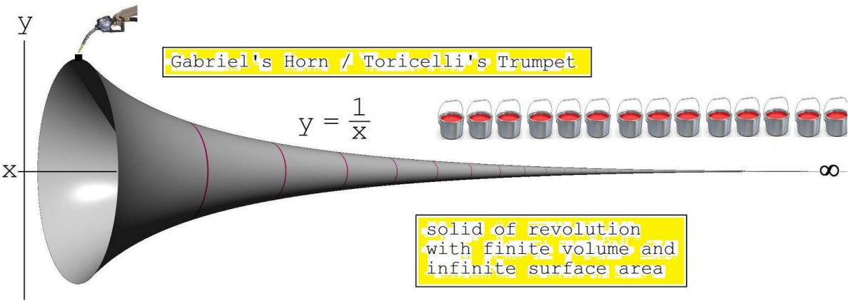
Figure 1. Gabriel's Horn / Toricelli's Trumpet.
