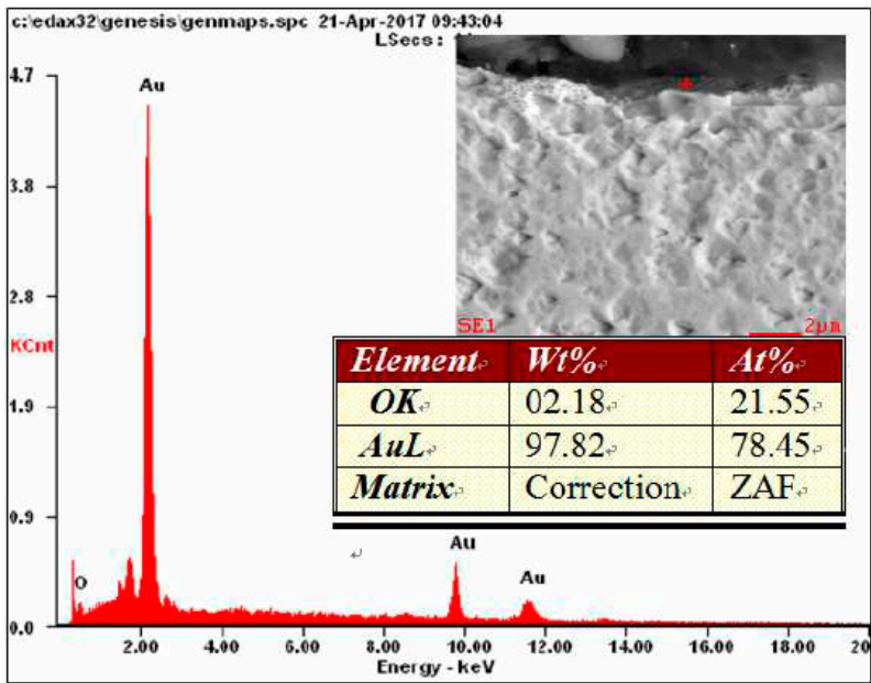
Figure 11. Results of microanalysis of the chemical composition of the Au electrode
