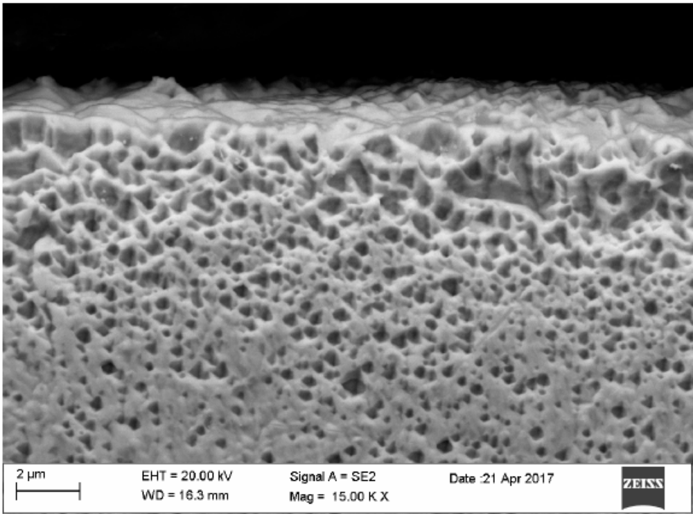
Figure 9. Surface of gold electrode
