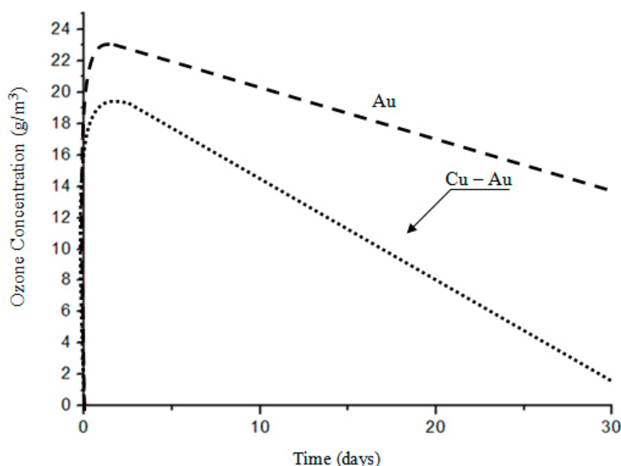
Figure 2. Dependence between ozone concentration and working time of electrodes
