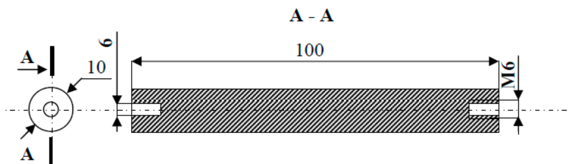
Figure 3. The shape and dimensions of the electrode made of gold
