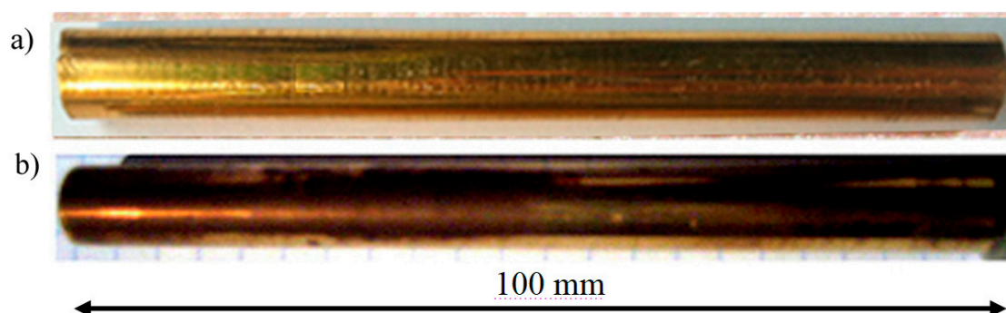
Figure 1. Photograph of electrodes after monthly use in a plasma reactor a) gold electrode, b) copper electrode galvanized coated with gold
