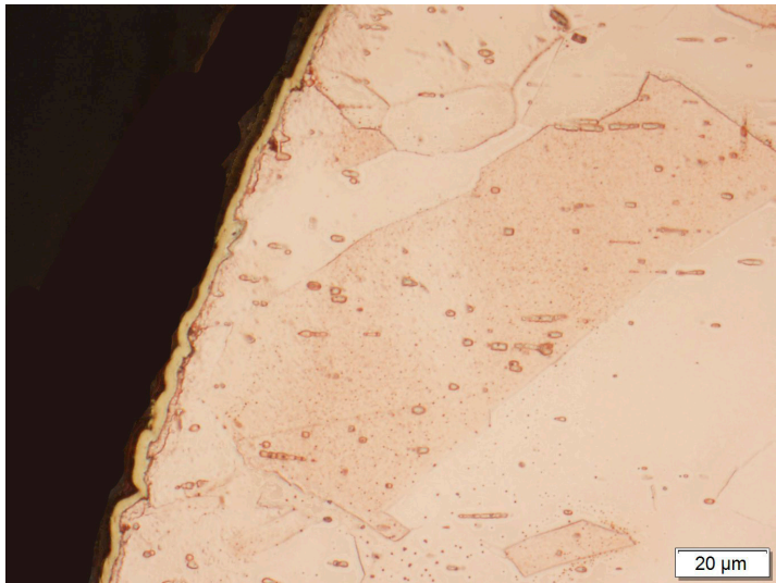
Figure 4. A gold layer applied galvanically to the surface of the copper electrode
