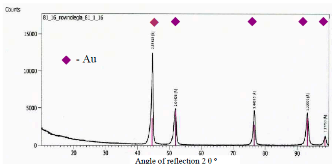
Figure 12. A diffractogram from the Au electrode surface
