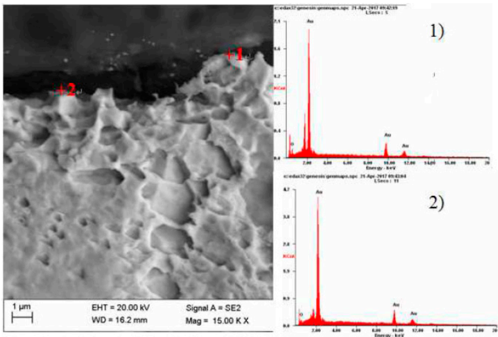
Figure 10. Results of microanalysis of the chemical composition of the Au electrode, from the areas marked in the photomicrographs
