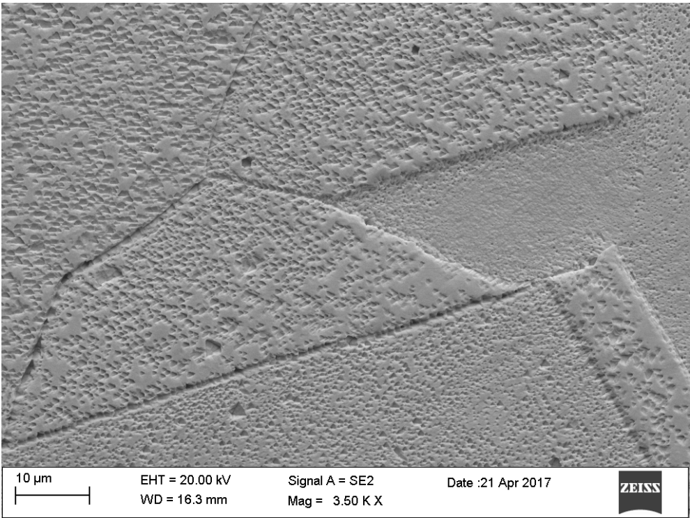
Figure 8. Large Au grains with twins in the structure
