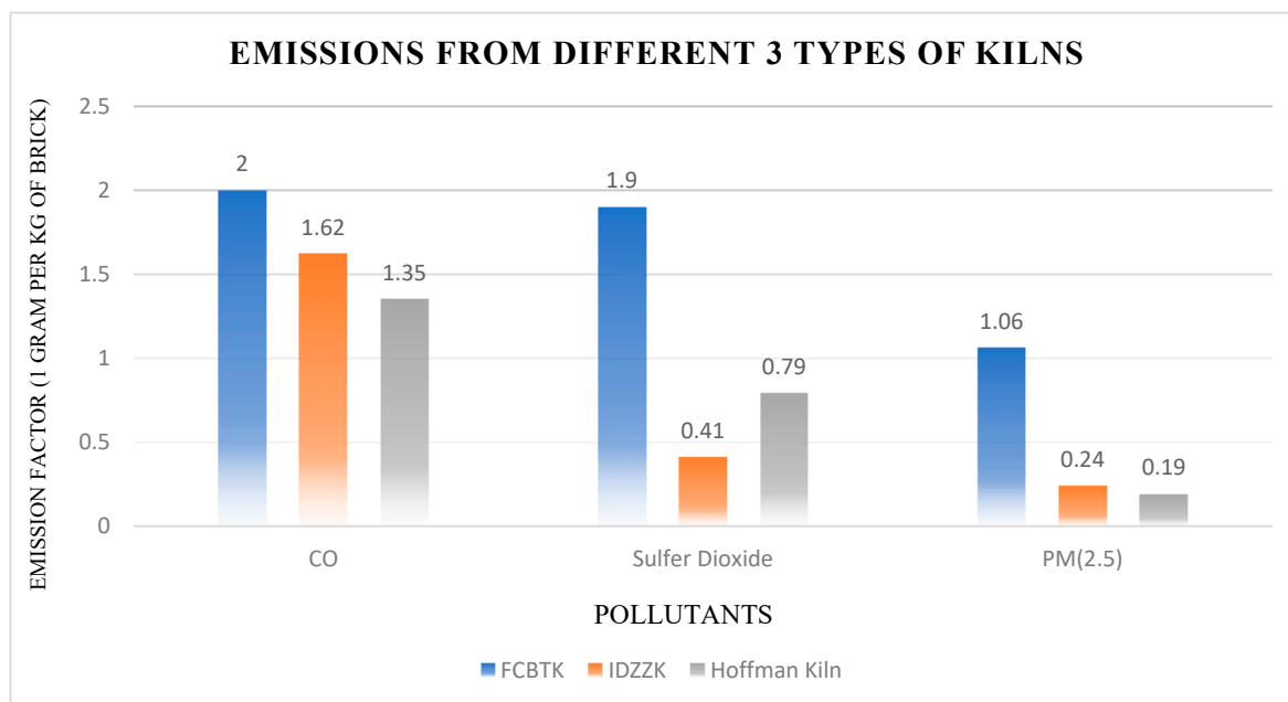
Figure 6. Comparison of emissions from 3 different types of brick kilns (Rauf et al., 2022). Carbon monoxide, sulfur oxide, and particulate matter emissions from the 3 different types of kilns including FCBTK, IDZZK, and Hoffman Kilns. Emissions given are per kg of brick production in each kiln.
