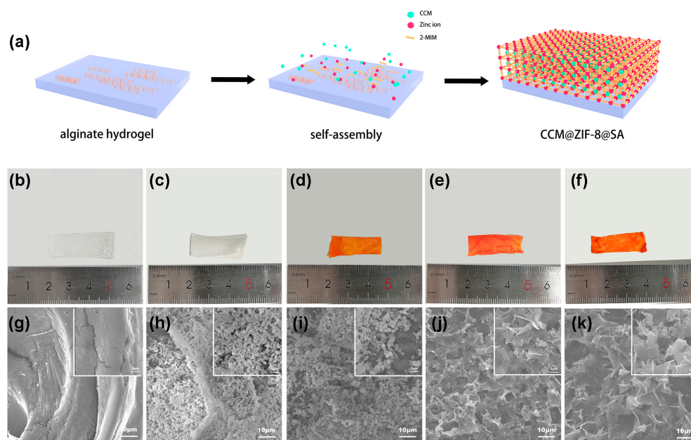
Figure 1. (a) Schematic diagram of the synthesis of a hydrogel, Optical photo of SA (b), ZIF-8@SA (c), 1CCM@ZIF-8@SA (d), 3CCM@ZIF-8@SA (e), 5CCM@ZIF-8@SA (f), SEM images of SA (g), ZIF-8 @SA (h), 1CCM@ZIF-8@SA (i), 3CCM@ZIF-8@SA (j), 5CCM@ZIF-8@SA (k).
