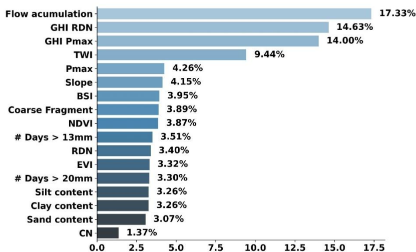
Figure 3. Relative importance (%) of predictor variables in the Random Forest (RF) model.
