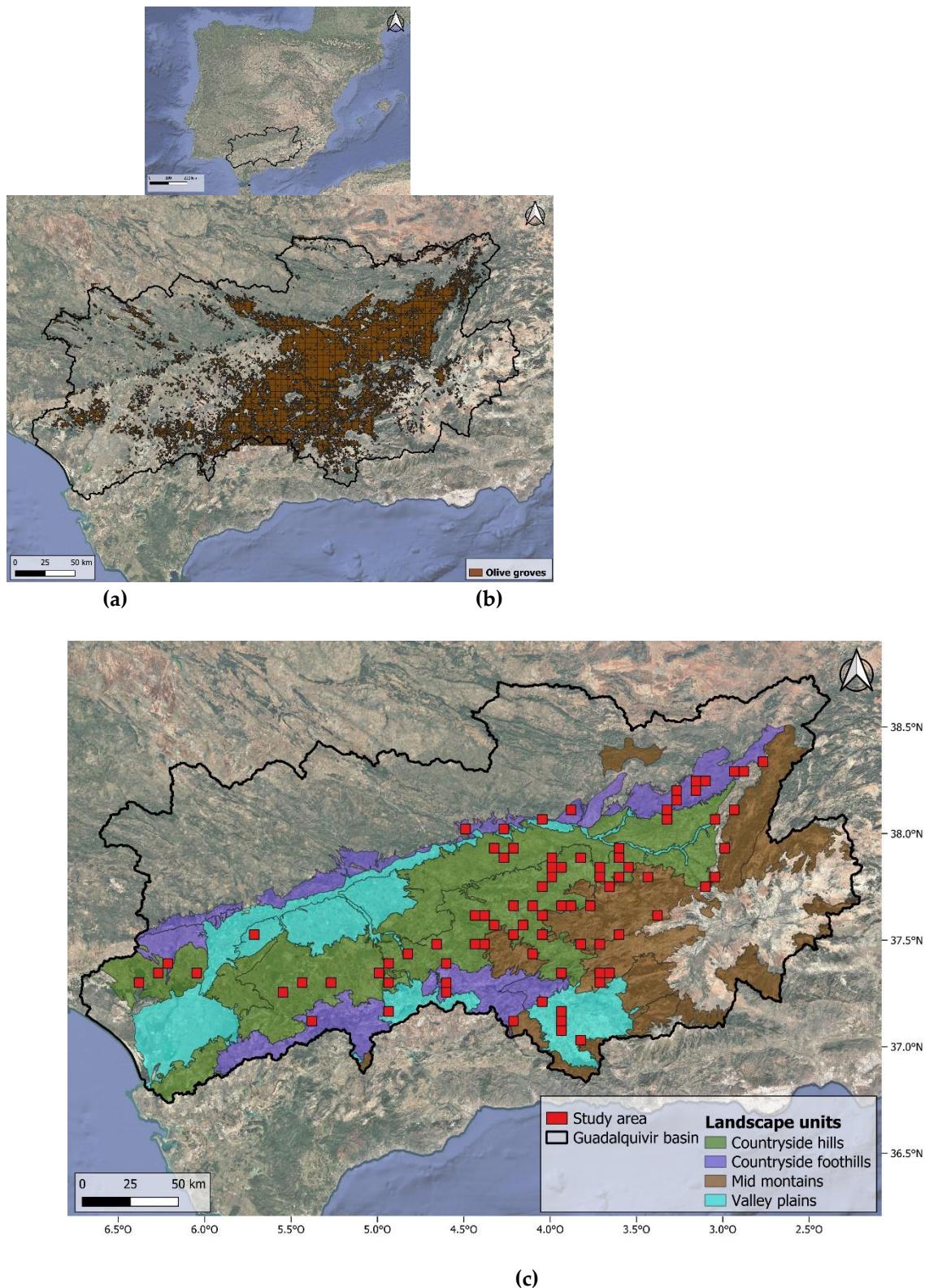
Figure 1. (a) Guadalquivir basin in Andalusia (Spain) (b) area occupied by olive groves in Andalusia obtained from Spanish Land Use Information System (SIOSE) (c) study area located in the principal landscapes units occupied by olive groves.
