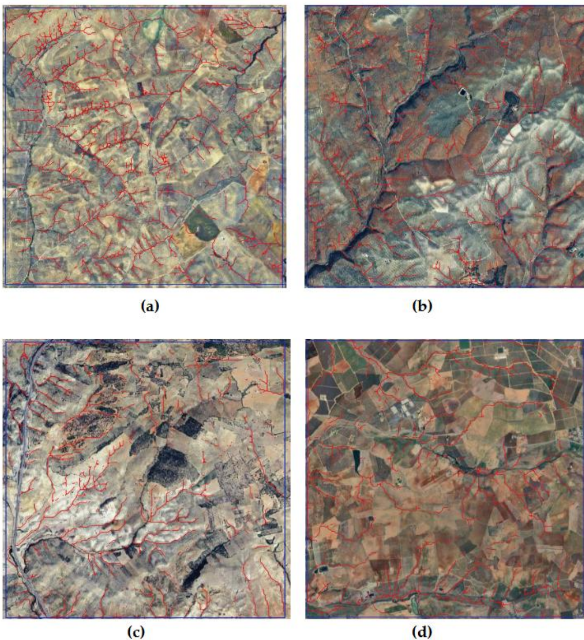
Figure 4. Examples of mapped gully network within four 25 km 2 study grid cells representing different landscape units: (a) Countryside hills; (b) Countryside foothills; (c) Mid mountains; (d) Valley plains.
