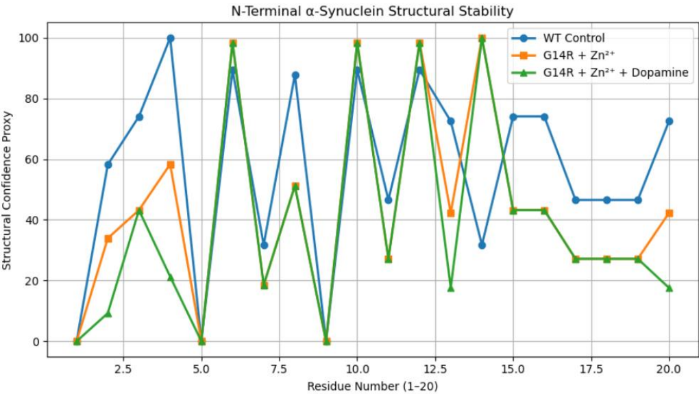
Figure 2. Residue-level structural confidence profiles for wild-type \alpha -synuclein, G14R under zinc-bound conditions, and G14R under combined zinc and dopamine conditions. Values represent normalized physicochemical confidence scores across residues 1–20.
