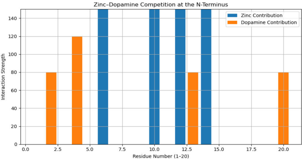
Figure 4. Zinc and dopamine contribution profile across the \alpha -synuclein N-terminus. Bars represent modeled interaction strengths for zinc and dopamine, illustrating residue-level overlap and competition.
