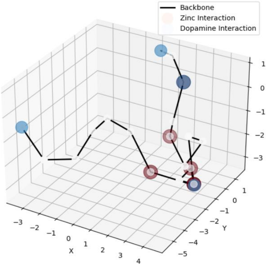
Figure 1. Coarse-grained three-dimensional model of the \alpha -synuclein N-terminus (residues 1–20). The backbone is represented as a random-coil approximation. Red spheres indicate relative zinc interaction strength, and blue spheres indicate relative dopamine interaction strength, scaled by modeled affinity.
