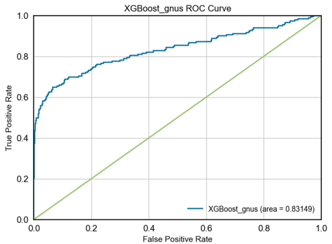
Figure 4. ROC curve diagram for XGBoost-GNUS.
