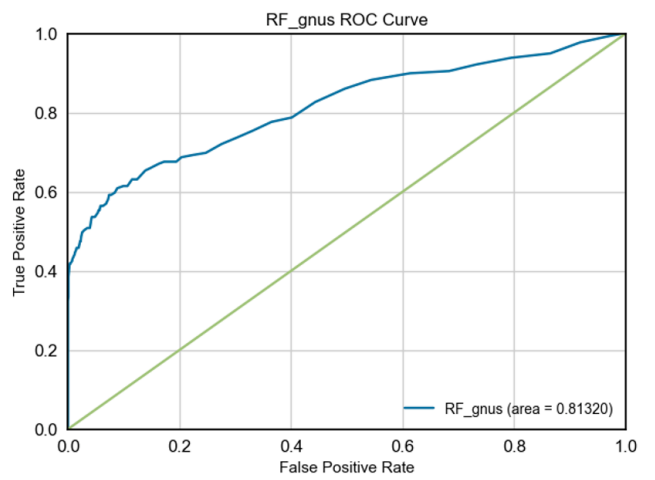
Figure 3. ROC curve diagram for RF-GNUS.
