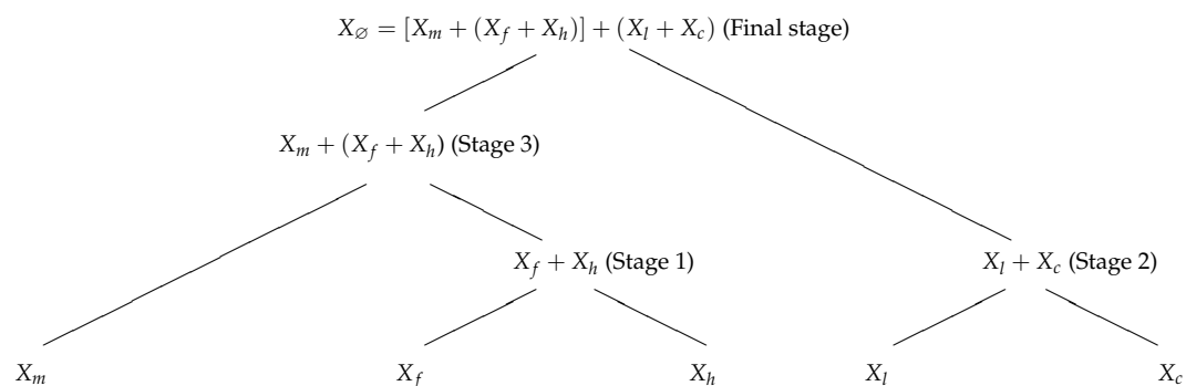
Figure 2. Hierarchical loss aggregation copula model for the gross (and net) loss ratio of the five business lines Motor, Fire, House, Liability and CTP, represented by X_m , X_f , X_h , X_l and X_c , respectively. The structure of the tree is determined by aggregating iteratively the two nodes with the strongest dependence.
