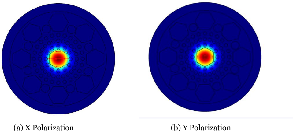
Figure 4. Light Confinement in the PCF-based oil detection of the Proposed sensor 's core.
