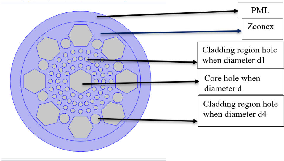
Figure 2. Designed View of Hollow Core-Based PCF sensor.
