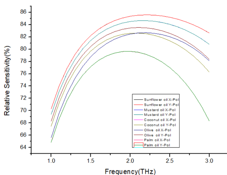
Figure 6. The relative sensitivity variation with frequency for different oil samples over the frequency ranging from 1.0 to 3.0 THz.
