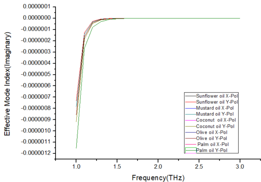
Figure 12. Change of effective refractive index with increasing frequency from 1.0 to 3.0 THz for different oil samples.
