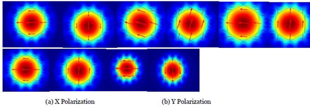
Figure 5. Light mode distribution of PCF-based oil detection of Proposed sensor.
