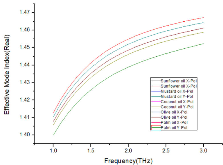
Figure 11. Change of effective refractive index with increasing frequency from 1.0 to 3.0 THz for different oil samples.
