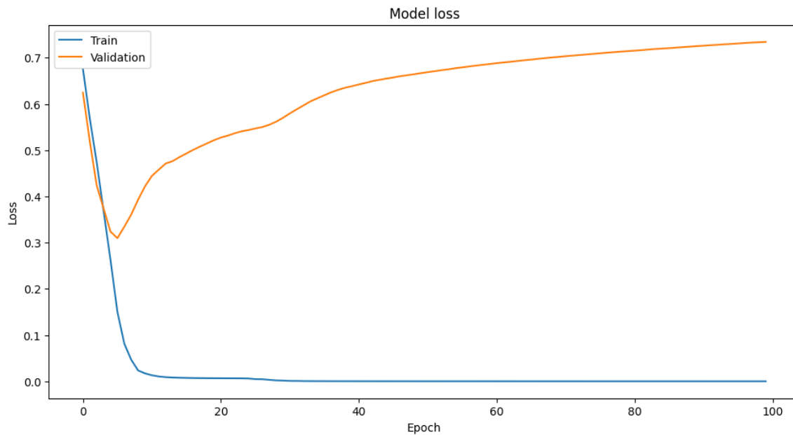
Fig. 2. Model Loss Graph: Observe the divergence at approximately epoch 10.
