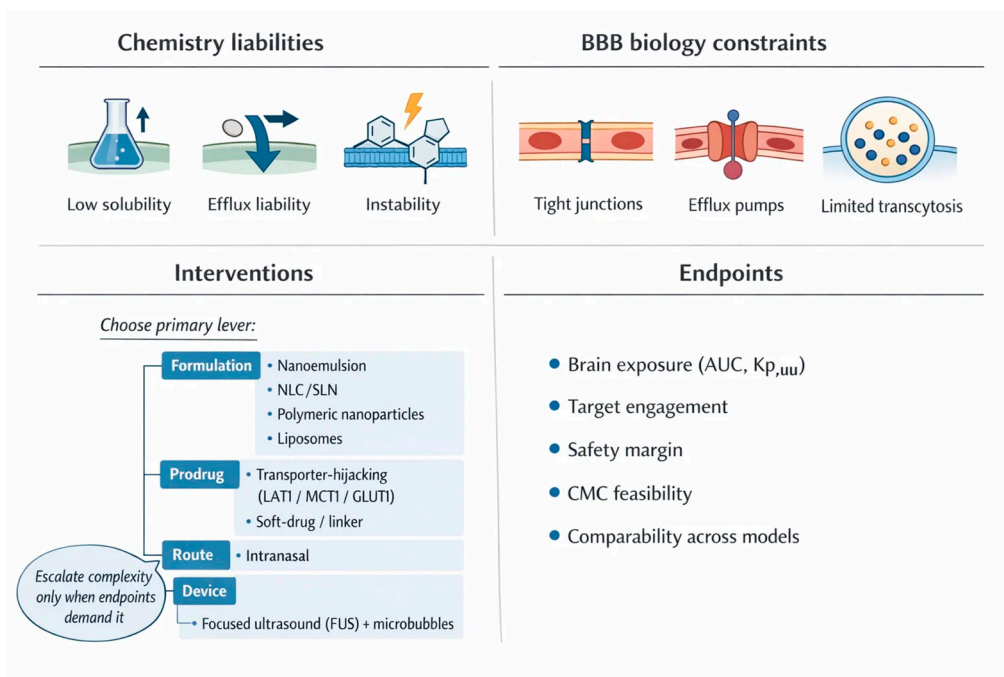
Figure 2. Decision tree for selecting CNS delivery strategies by payload liabilities and clinical context. The schematic provides a pragmatic decision tree to match a CNS payload to the most efficient delivery strategy. The workflow begins with dominant liabilities: (i) solubility/dissolution limitation, (ii) efflux liability (e.g., P-gp/BCRP/MRPs), and (iii) chemical or metabolic instability. Solubility-driven failure routes first to formulation solutions (solubilizing vehicles, lipid systems, polymeric nanoparticles, mucoadhesive/intranasal formats when appropriate). Predominant efflux liability routes to prodrug design (efflux-evading promoieties or transporter-hijacking approaches such as GLUT1/LAT1/MCT1) and/or carrier shielding/targeting (stealth/corona control; RMT ligands such as TfR/LRP1). Instability-driven failure routes to protective encapsulation or stability-optimized prodrugs with controlled release. Clinical context modifiers (need for rapid onset, diffuse vs focal pathology, and tolerability constraints) direct selection of route (e.g., intranasal bypass) or focused ultrasound (FUS) + microbubbles for localized BBB modulation. Each terminal node specifies decision-grade endpoints: brain exposure (AUC, K_{p,brain} , K_{p,uu} ), target engagement, safety margin, and CMC scalability. AUC, area under the curve; BBB, blood–brain barrier; BCRP, breast cancer resistance protein; CMC, chemistry, manufacturing, and controls; CNS, central nervous system; FUS, focused ultrasound; GLUT1, glucose transporter 1; K_{p,brain} , brain-to-plasma partition coefficient; K_{p,uu} , unbound brain-to-plasma partition coefficient; LAT1, L-type amino acid transporter 1; MCT1, monocarboxylate transporter 1; MRPs, multidrug resistance–associated proteins; P-gp, P-glycoprotein; RMT, receptor-mediated transcytosis; TfR, transferrin receptor; LRP1, low-density lipoprotein receptor–related protein 1.
