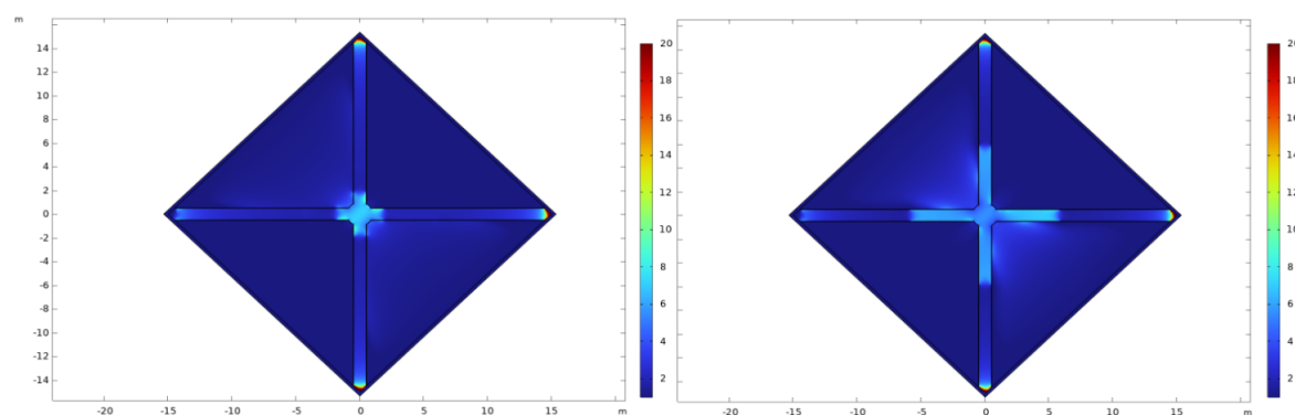
Figure 5. Shielding factor achieved by covering the interferometer arms with a 2mm-thick layer of a ferromagnetic layer with a relative magnetic permeability of 100,000 over lengths of 1 meter (left figure) and 5 meters (right figure), respectively. The external uniform magnetic field is at 45^\circ with respect to the interferometer arms.
