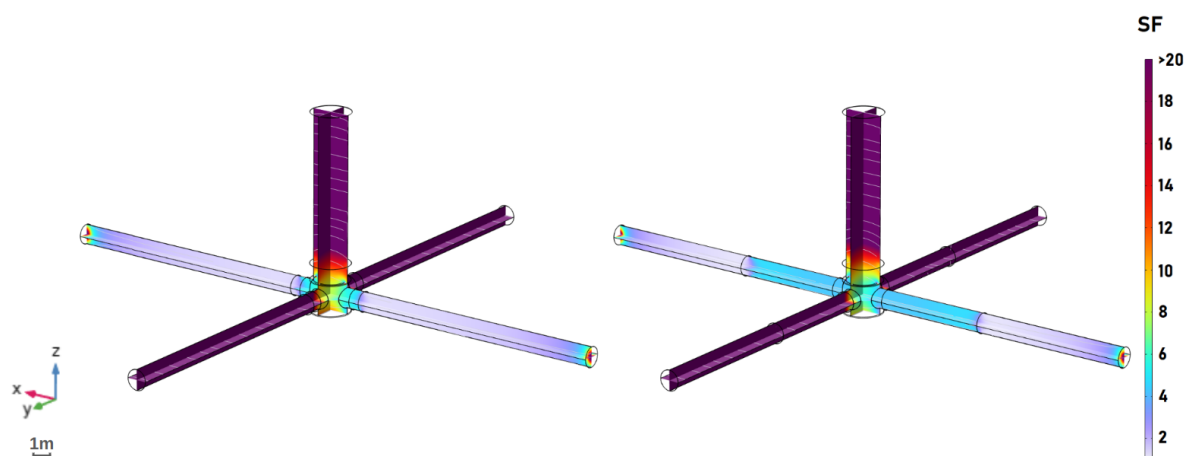
Figure 4. Shielding factor achieved by covering the interferometer arms with a 2mm-thick layer of a ferromagnetic layer with a relative magnetic permeability of 100,000 over lengths of 1 meter (left figure) and 5 meters (right figure), respectively. The external uniform magnetic field is directed along one arm of the interferometer.
