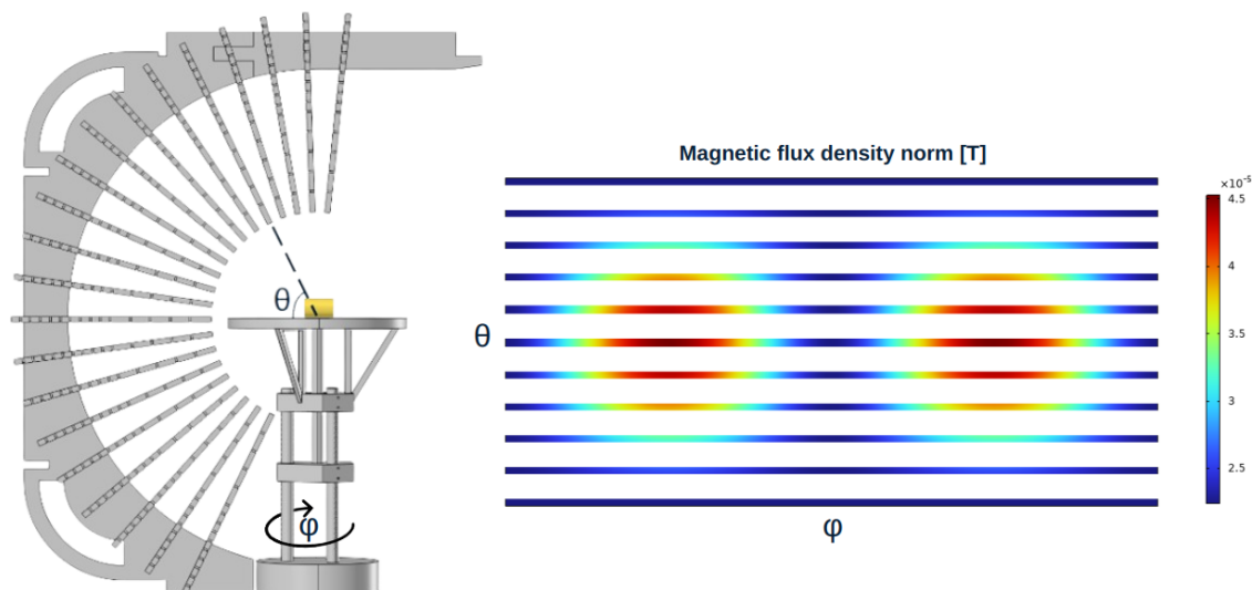
Figure 3. Simulation of the magnetic field of an ideal dipole as it will be observed by MANET.
