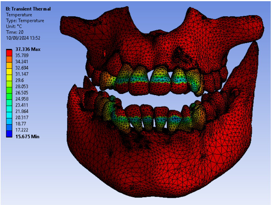
Figure 14. Thermal map.
