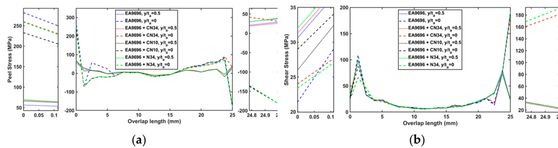
Figure 7. (a) peel and (b) shear stresses distributions in EA9696 adhesively bonded joints at room temperature, respectively.
