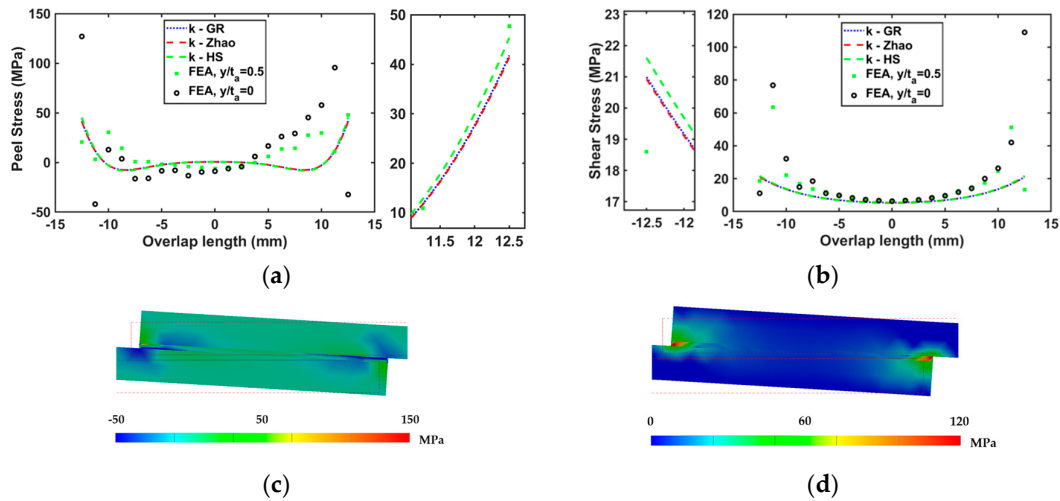
Figure 9. Comparison of (a) peel and (b) shear stresses distributions under 240 N/mm between finite element analysis (FEA) and Goland and Reissner (GR) theory results at the interface and mid-section of 10 wt.% TEPs-epoxy adhesive bondline. (c) peel and (d) shear stresses distributions in FEA. *k-HS [29] and k-Zhao [30] refer to the bending moment factors, which were calculated based on their respective solutions.
