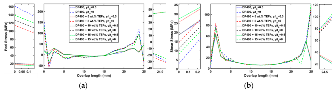
Figure 5. (a) peel and (b) shear stresses distributions in DP490 adhesively bonded joints at room temperature, respectively.
