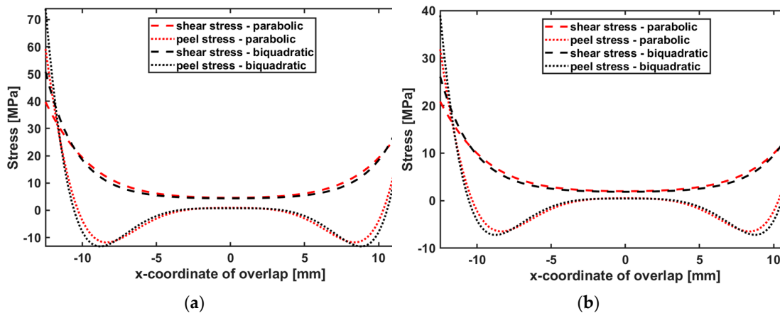
Figure 14. Stress distribution of EA9696 adhesive joints (a) at room temperature and (b) at 100°C.
