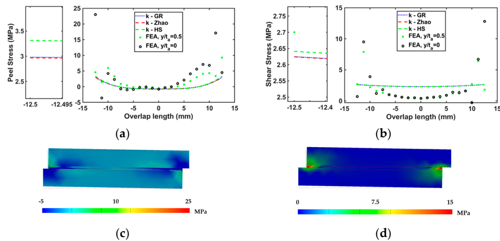
Figure 10. Comparison of (a) peel and (b) shear stresses distributions under 60 N/mm between finite element analysis (FEA) and Goland and Reissner (GR) theory results at the interface and mid-section of 10 wt.% TEPs-epoxy adhesive bondline at 145°C. (c) peel and (d) shear stresses distributions in FEA. *k-HS [29] and k-Zhao [30] refer to the bending moment factors, which were calculated based on their respective solutions.
