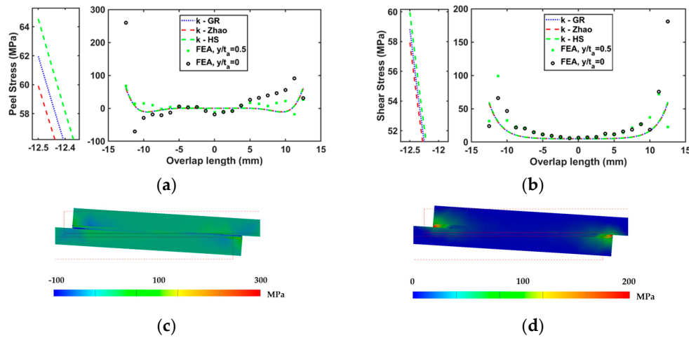
Figure 11. Comparison of (a) peel and (b) shear stresses distributions under 300 N/mm between finite element analysis (FEA) and Goland and Reissner (GR) theory results at the interface and mid-section of CN34 interleaved epoxy adhesive bondline. (c) peel and (d) shear stresses distributions in FEA. *k-HS [29] and k-Zhao [30] refer to the bending moment factors, which were calculated based on their respective solutions.
