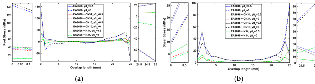
Figure 8. (a) peel and (b) shear stresses distributions in EA9696 adhesively bonded joints at 100°C, respectively.
