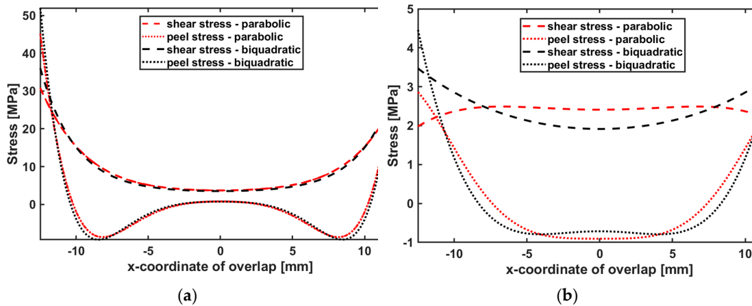
Figure 13. Stress distribution of DP490 adhesive joints (a) at room temperature and (b) at 145°C.
