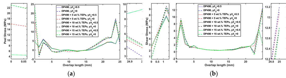
Figure 6. (a) peel and (b) shear stresses distributions in DP490 adhesively bonded joints at 145°C, respectively.
