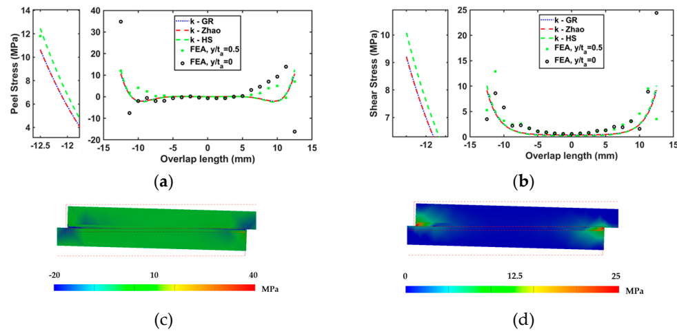
Figure 12. Comparison of (a) peel and (b) shear stresses distributions under 40 N/mm between finite element analysis (FEA) and Goland and Reissner (GR) theory results at the interface and mid-section of CN34 interleaved epoxy adhesive bondline at 100°C. (c) peel and (d) shear stresses distributions in FEA. *k-HS [29] and k-Zhao [30] refer to the bending moment factors, which were calculated based on their respective solutions.
