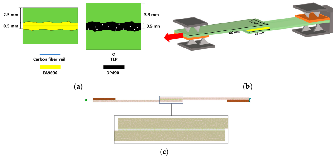
Figure 4. (a), (b) the single lap joint with details of geometry and boundary conditions and (c) the representative mesh used for the stress analysis.
