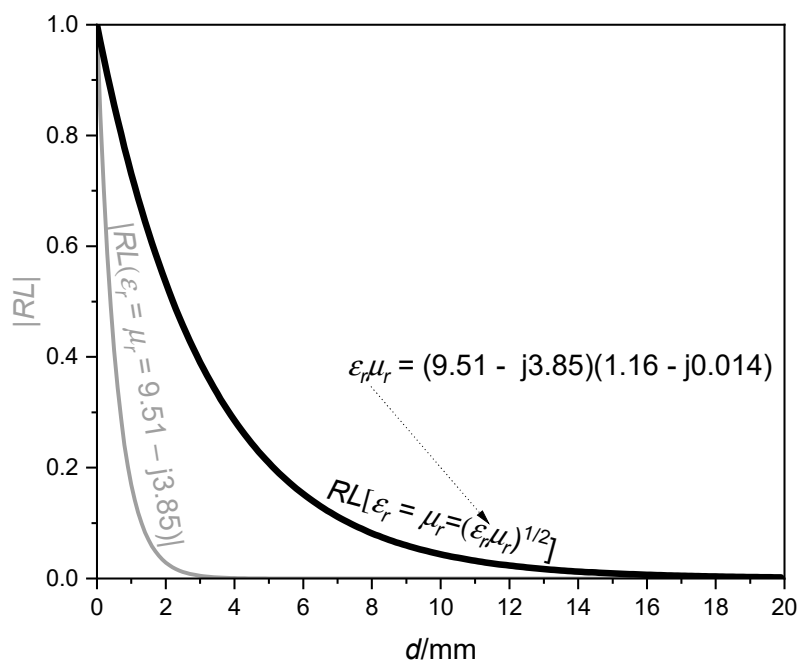
Figure 4. |RL| calculated by Eq. Error! Reference source not found. or Error! Reference source not found. with \epsilon_r = \mu_r = 9.51 - j3.85 and \epsilon_r = \mu_r = [(9.51 - j3.85)(1.16 - j0.014)]^{1/2} at 11 GHz. [10].
