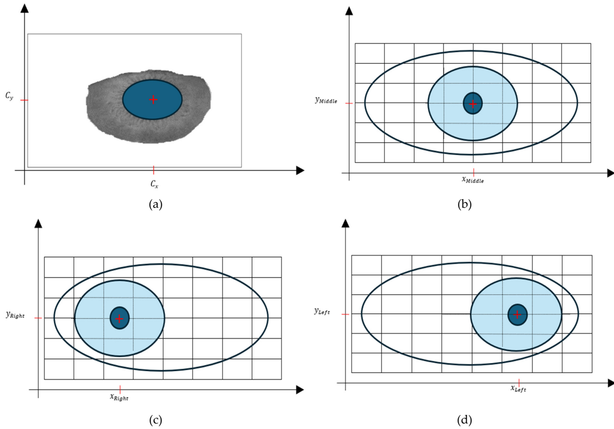
Figure 6. The coordinates representing each direction, (a) the iris center coordinates ( C_x , C_y ), (b) the Middle direction, (c) the Right direction, and (d) the Left direction.
