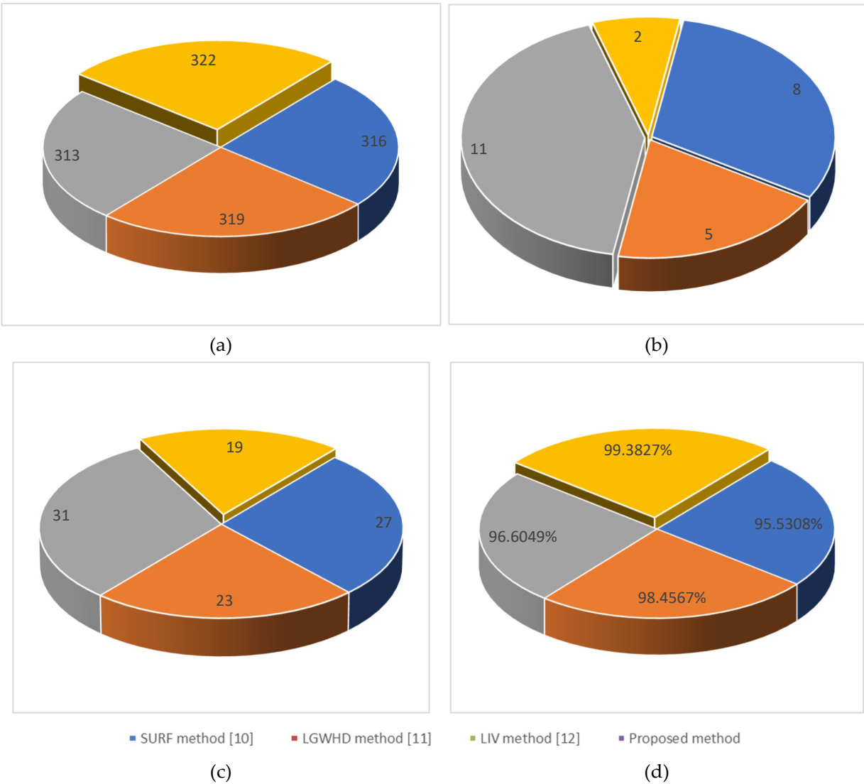
Figure 10. Iris recognition evaluation results, (a) True positive, (b) False positive, (c) False negative, and (d) Iris recognition rate.
