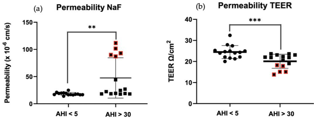
Figure 4. Membrane permeability measurement of HBEC-5i after 5 hours of 10 \mu\text{g} exosomes from patients without OSAS AHI < 5 vs. patients with OSAS AHI > 30. (A) NaF: sodium fluorescein - results are represented as mean value \pm s.e.m (n=15 triplicate) **p=0.0049<0.01 between AHI < 5 vs. AHI > 30. (B) TEER: transendothelial electrical resistance - results are represented as mean value \pm s.e.m (n=15 triplicate) ***p=0.0009<0.01 between AHI < 5 vs AHI > 30.
