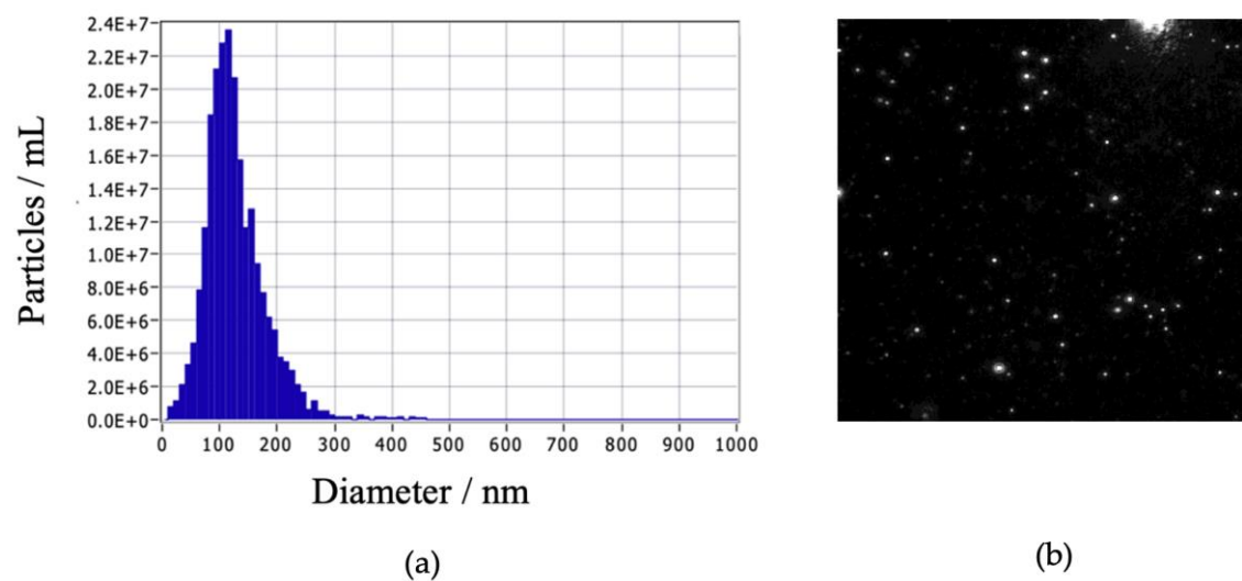
Figure 1. Characterization of exosomes using NTA zeta sizer instrument. (A) Particles in mL as a function of diameter in nm, (B) Visualization of exosomes.
