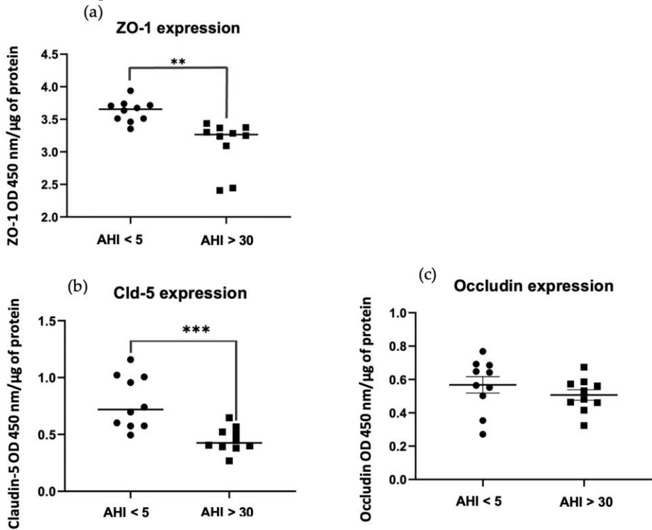
Figure 5. Whole cell ELISA assay. Results are represented as mean value \pm s.e.m (n=10 triplicate). Expressions of ZO-1(A) **p=0.001<0.01 , claudin-5 (B) ***p=0.0008<0.01 , and occludin (C) p=0.3126>0.01 proteins after exposure of HBEC-5i 5 hours of 10 \mu\text{g} exosomes from patients without OSAS AHI < 5 vs. patients with OSAS AHI > 30.
