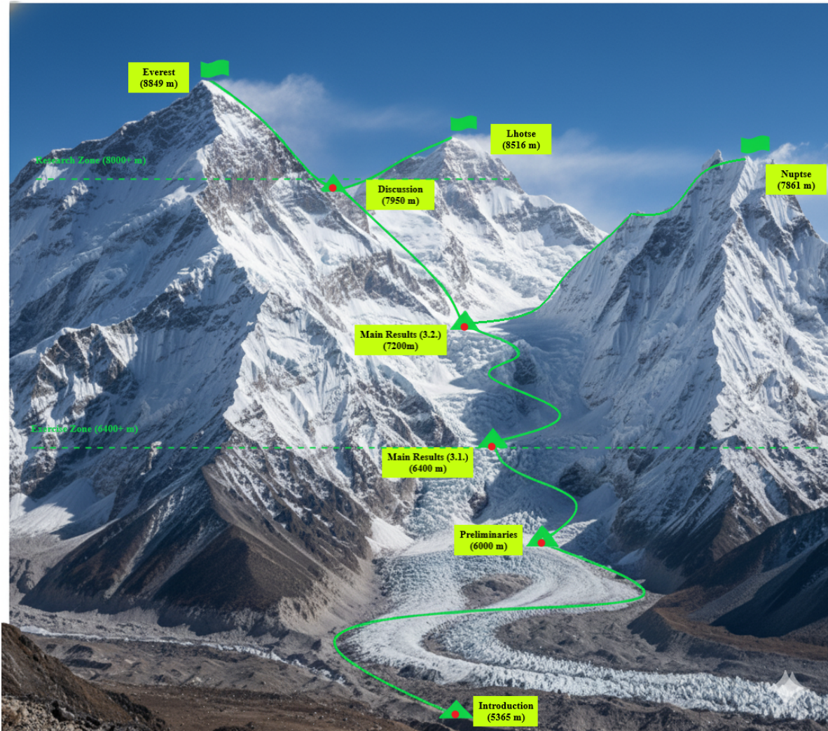
Figure 1. Everest analogy for the paper’s structure: the route begins at Introduction , traverses the glacier of Preliminaries , reaches Camp 2 at 6,400 m ( Main Results 3.1 ), climbs to 7,200 m ( Main Results 3.2 ), pauses near 7,950 m ( Discussion ), and enters the 8,000+ m Research Zone , with summits at Everest (8,849 m) and Lhotse (8,516 m).
