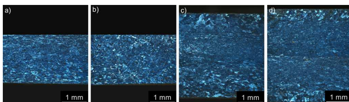
Figure 6. LOM images of materials after annealing 300 °C / 30 min, 450 °C / 30 min and one CGP cycle performed at 300 °C: (a) AlLi MC, (b) AlLiSc MC, (c) AlLi TRC and (d) AlLiSc TRC.
