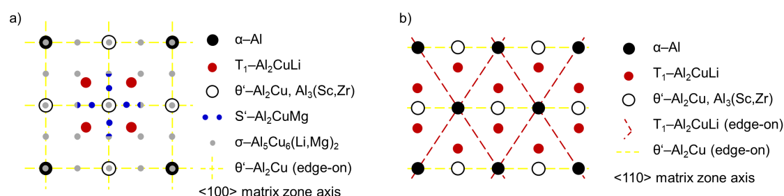
Figure 18. Schematic diagrams of the diffraction pattern along: (a) \langle 100 \rangle , (b) \langle 110 \rangle zone axes.
