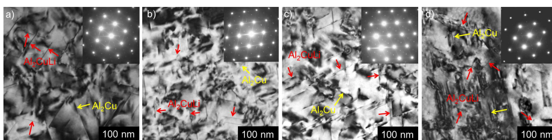
Figure 21. TEM micrograph of materials after annealing 300 °C / 30 min, 450 °C / 30 min, one CGP cycle performed at 300 °C, solution treatment 530 °C / 30 min, 3 % pre-straining and aging 180 °C / 14 h (near peak age condition), zone [110]: (a) AILi MC, (b) AILiSc MC, (c) AILi TRC and (d) AILiSc TRC.
