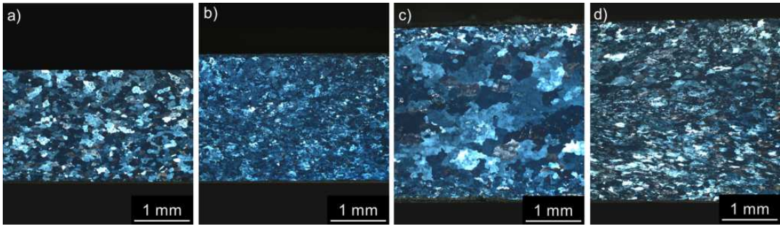
Figure 11. LOM images of materials after annealing 300 °C / 30 min, 450 °C / 30 min, one CGP cycle and solution treatment 530 °C / 30 min: (a) AlLi MC, (b) AlLiSc MC, (c) AlLi TRC and (d) AlLiSc TRC.
