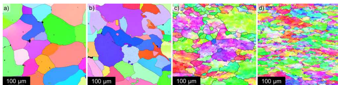
Figure 4. EBSD inverse pole figures of as-cast materials: (a) AlLi MC, (b) AlLiSc MC, (c) AlLi TRC and (d) AlLiSc TRC. Central parts of strips were selected in the TRC materials.
