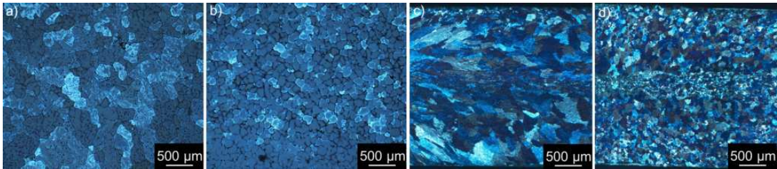
Figure 1. LOM images of the as-cast materials showing grain distributions in: (a) AILi MC, (b) AILiSc MC, (c) AILi TRC and (d) AILiSc TRC.
