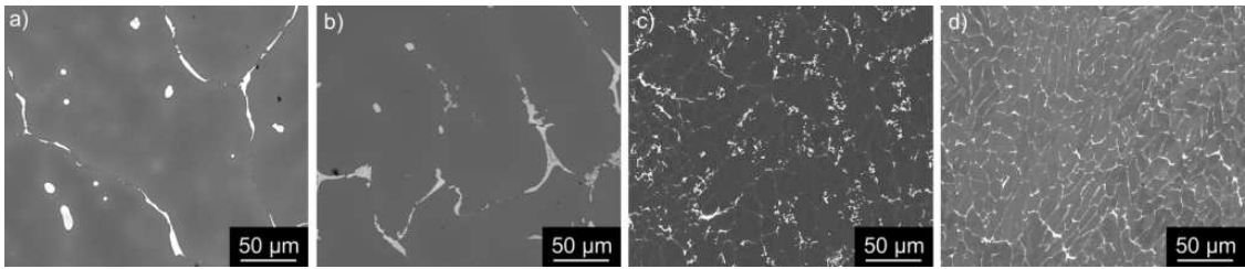
Figure 2. SEM BSE images of eutectic cells in as-cast materials: (a) AILi MC, (b) AILiSc MC, (c) AILi TRC and (d) AILiSc TRC, demonstrating a positive influence of TRC and Sc addition on the refinement of the structure.
