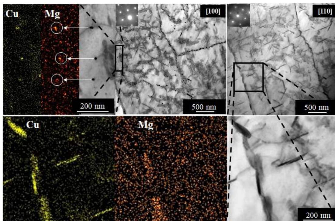
Figure 19. TEM images showing the same area in [100] and [110] orientations and corresponding EDS maps of needle-shaped subgrain boundary particles containing Cu and Mg.
