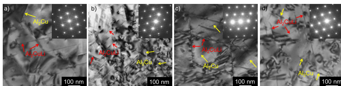
Figure 17. TEM micrograph of materials after annealing 300 °C / 30 min, 450 °C / 30 min, one CGP cycle performed at 300 °C, solution treatment 530 °C / 30 min and aging 180 °C / 40 h (near peak age condition), zone [110]: (a) AlLi MC, (b) AlLiSc MC, (c) AlLi TRC and (d) AlLiSc TRC.
