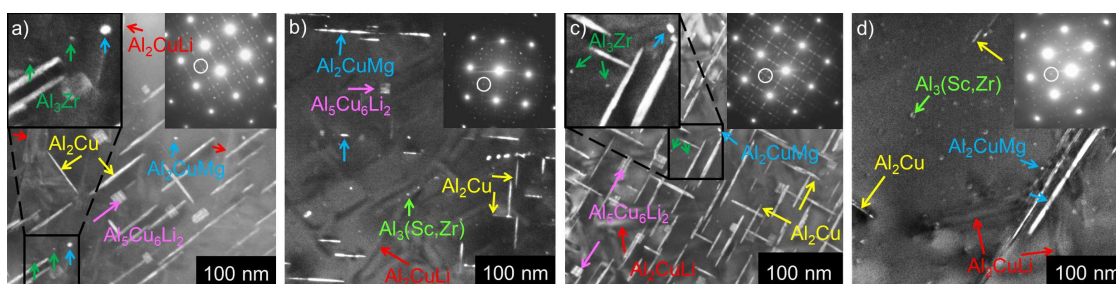
Figure 16. TEM micrograph of materials after annealing 300 °C / 30 min, 450 °C / 30 min, one CGP cycle performed at 300 °C, solution treatment 530 °C / 30 min and aging 180 °C / 40 h (near peak age condition), dark field, zone [001] : (a) AILi MC, (b) AILiSc MC, (c) AILi TRC and (d) AILiSc TRC. Small \text{Al}_3\text{Zr} particles are highlighted in insets in a) and c).
