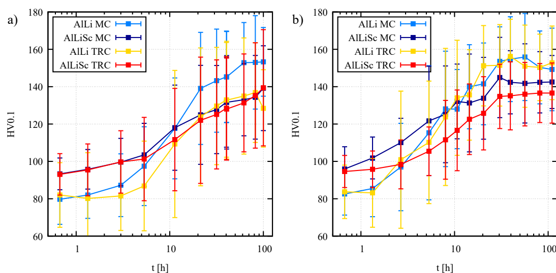
Figure 13. Microhardness evolution during aging: (a) specimen without pre-straining after the solution treatment, (b) specimen pre-strained by 3 % after the solution treatment.
