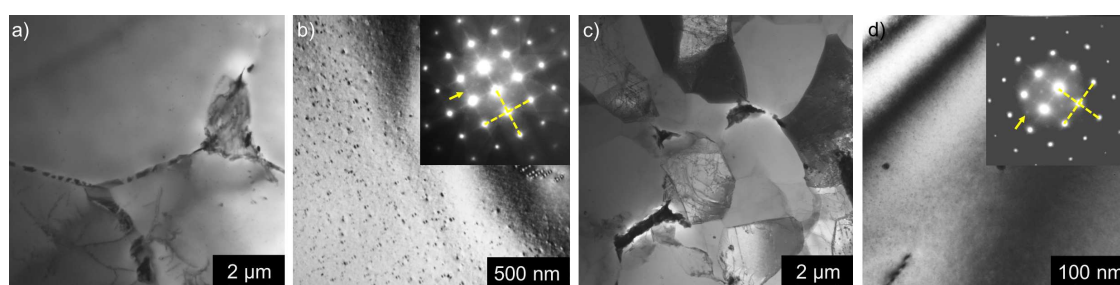
Figure 5. TEM micrographs of the as-cast AlLiSc materials: (a,b) MC, (c,d) TRC. Both the yellow arrows in b,d) pointing at the position of the superstructural spots and streaks highlighted by the yellow dashed lines reflects the presence of fine \theta' - \text{Al}_2\text{Cu} precipitates.
