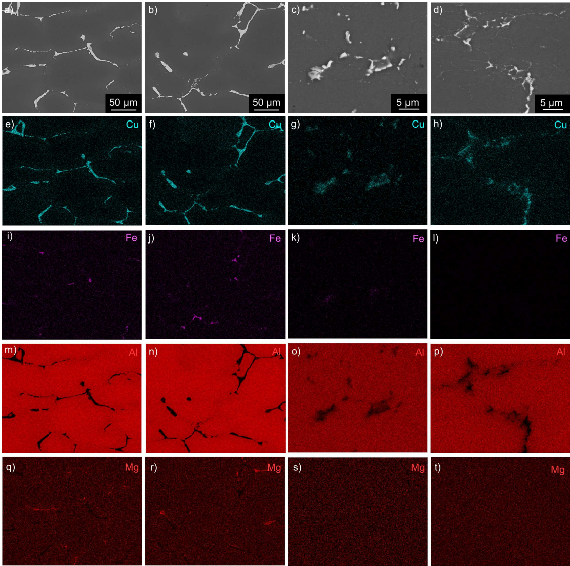
Figure 9. SEM BSE images and corresponding EDS maps of materials after annealing 300 °C / 30 min, 450 °C / 30 min and one CGP cycle performed at 300 °C: (a) AlLi MC, (b) AlLiSc MC, (c) AlLi TRC and (d) AlLiSc TRC.
