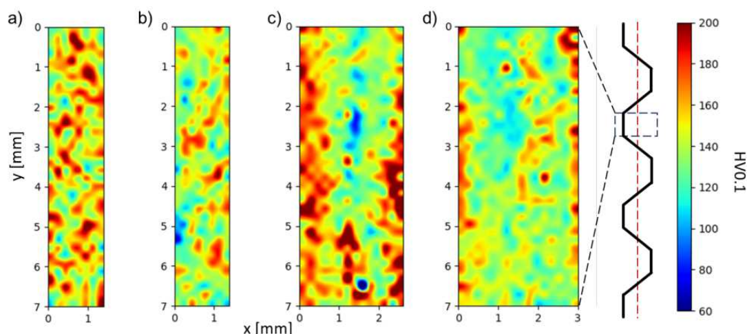
Figure 14. Distribution of microhardness through the sample thickness of materials after annealing 300 °C / 30 min, 450 °C / 30 min, one CGP cycle performed at 300 °C, solution treatment 530 °C / 30 min, 3 % pre-straining and aging 180 °C / 110 h: (a) AILi MC, (b) AILiSc MC, (c) AILi TRC and (d) AILiSc TRC.
