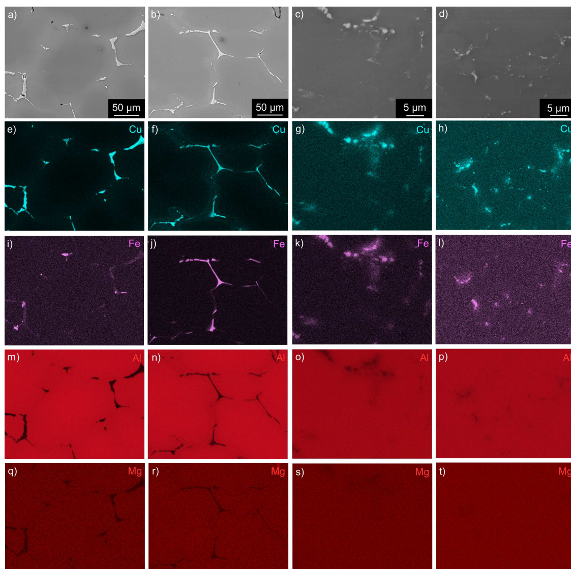
Figure 10. SEM BSE images and corresponding EDS maps of materials after annealing 300 °C / 30 min, 450 °C / 30 min, one CGP cycle and solution treatment 530 °C / 30 min: (a) AILi MC, (b) AILiSc MC, (c) AILi TRC and (d) AILiSc TRC.
