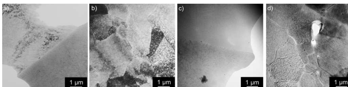
Figure 20. TEM micrographs of boundaries in materials after annealing 300 °C / 30 min, 450 °C / 30 min, one CGP cycle performed at 300 °C, solution treatment 530 °C / 30 min, 3 % pre-straining and aging 180 °C / 14 h (near peak age condition), bright field: (a) AILi MC, (b) AILiSc MC, (c) AILi TRC and (d) AILiSc TRC.
