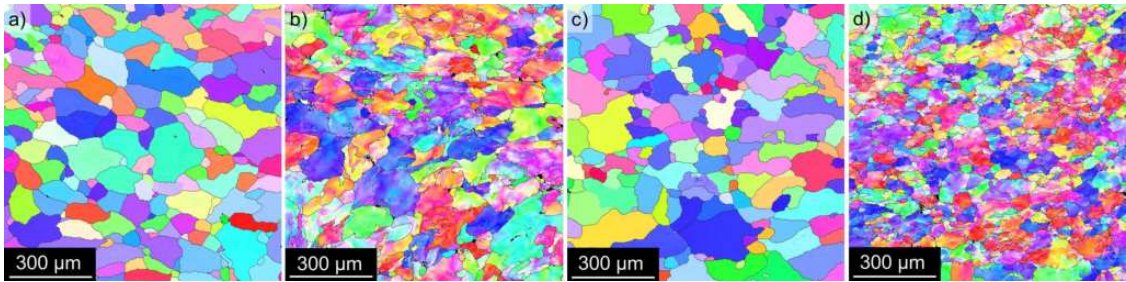
Figure 12. EBSD IPF maps of materials after annealing 300 °C / 30 min, 450 °C / 30 min, one CGP cycle and solution treatment 530 °C / 30 min: (a) AlLi MC, (b) AlLiSc MC, (c) AlLi TRC and (d) AlLiSc TRC.
