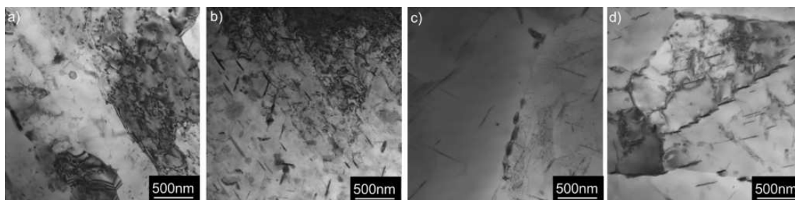
Figure 8. TEM micrographs showing the distribution of Cu and Mg-rich particles in materials after annealing 300 °C / 30 min, 450 °C / 30 min and one CGP cycle performed at 300 °C: (a) ALi MC, (b) ALiSc MC, (c) ALi TRC and (d) ALiSc TRC.
