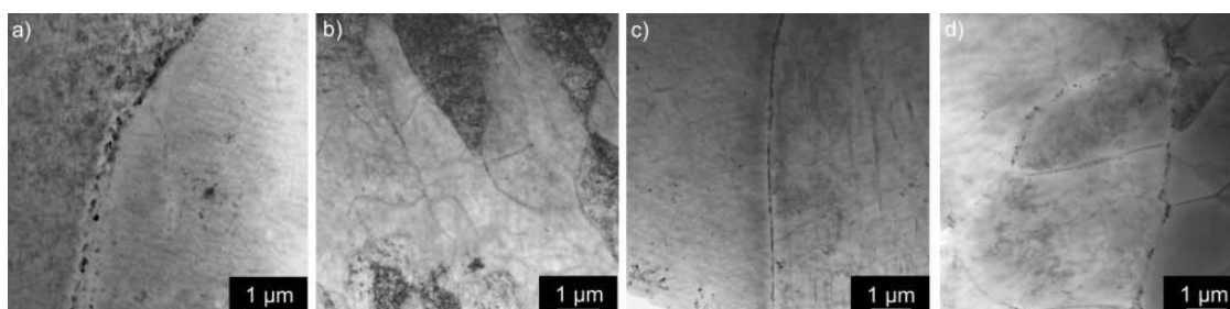
Figure 15. TEM micrograph of materials after annealing 300 °C / 30 min, 450 °C / 30 min, one CGP cycle performed at 300 °C, solution treatment 530 °C / 30 min and aging 180 °C / 40 h: (a) AILi MC, (b) AILiSc MC, (c) AILi TRC and (d) AILiSc TRC.
