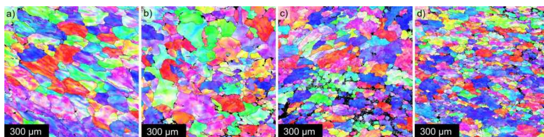
Figure 7. EBSD IPF maps of materials after annealing 300 °C / 30 min, 450 °C / 30 min and one CGP cycle performed at 300 °C: (a) AlLi MC, (b) AlLiSc MC, (c) AlLi TRC and (d) AlLiSc TRC.
