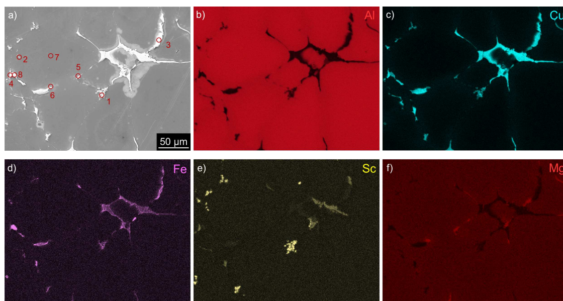
Figure 3. BSE image with corresponding EDS maps showing the distribution of Al, Cu, Fe, Sc, and Mg in a selected zone containing rare Sc-rich particles in the MC AlLiSc alloy in the as-cast state.
