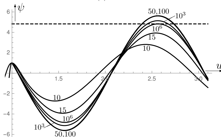
Figure 4. Solutions of Eq (67) to the initial conditions (68) for small values of \beta ( =10, 15, \dots, 10^6 ). For \beta=10 and 15, the solution curves start shortly before u=1 so that their parabolic curvature at \beta=1 becomes visible. The amplitude of the curves increases for \beta < \approx 50 and decreases in turn for larger \beta . Already for \beta=10^6 essentially the curve (81), calculated below for \beta=2.79 \cdot 10^{122} , is obtained.
