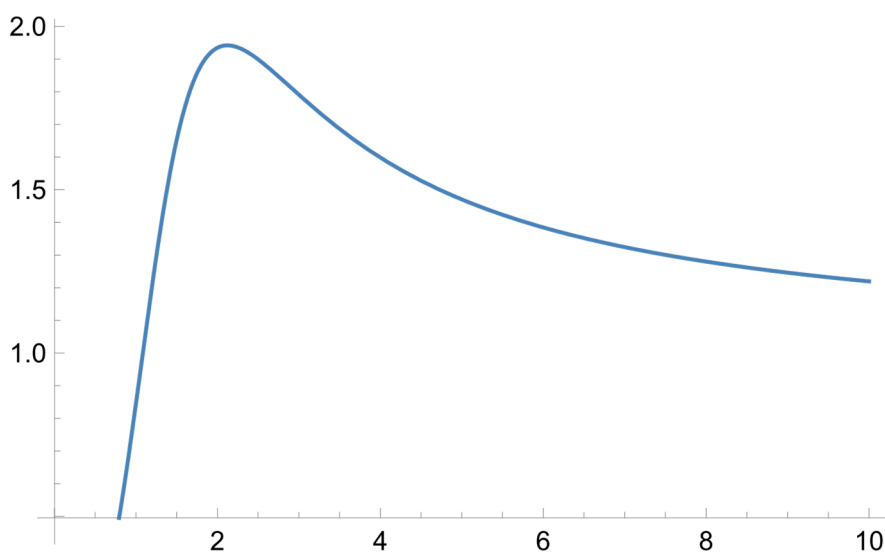
Figure 4.10. Interaction II. The function y = \frac{v^2(x)}{\sigma} if k = 0.5 . Source: Figure by author.
