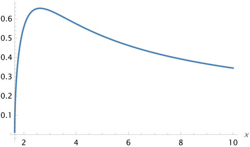
Figure 1.1. Interaction IV. The graph of the function y = \frac{v(x)}{\sqrt{\sigma}} , if k = -1 , for small values of x . Source: Figure by author.
