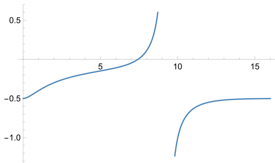
Figure 4.14. Interaction II. The function y = \frac{V(x)}{\sigma} if k = 0.1 . Source: Figure by author.
