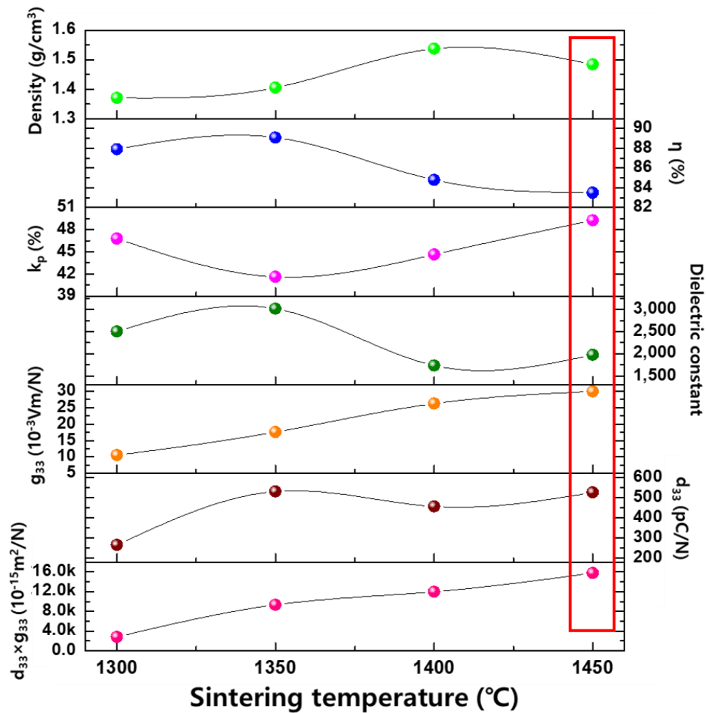
Fig. 2 Piezoelectric and dielectric properties of the BCTZC 0.3 ceramics sintered at various temperatures.
