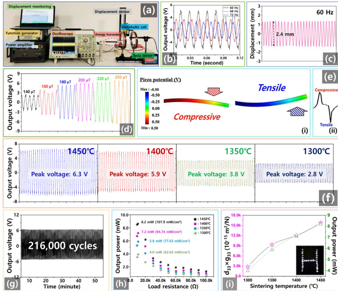
Fig. 3 (a) Photograph of the experimental environment used to observe the power-generation characteristics of the LPEH in various magnetic fields ( \mu\text{T} ). (b) Open-circuit output voltage (V) of the LPEH at various frequencies. (c) Displacement of the LPEH at a resonance frequency of 60 Hz. (d) Open-circuit output voltage (V) of the LPEH in differential magnetic fields ( \mu\text{T} ). (e) Simulated data of the piezoelectric potential (V) when stress is applied. (f) Open-circuit output voltage (V) characteristics of LPEHs composed of BCTZC 0.3 films processed at various sintering temperatures ( ^{\circ}\text{C} ). (g) Open-circuit output voltage of the LPEH for a durability test of over 216,000 cycles performed in a magnetic field of 250 \mu\text{T} . (h) Instantaneous maximum output power (mW) values of LPEHs with BCTZC 0.3 films sintered at various temperatures ( ^{\circ}\text{C} ) under specific load resistances ( \Omega ) for impedance matching. (i) Power conversion constant ( d_{33} \times g_{33} ) and instantaneous maximum output power (mW) values of LPEHs with BCTZC 0.3 films depending on their sintering temperatures ( ^{\circ}\text{C} ). The inset shows lighting when using 30 white light-emitting diodes.
