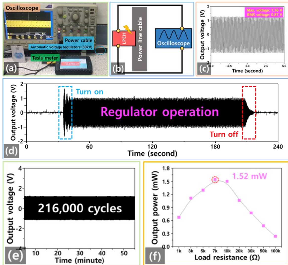
Fig. 5 (a) Experimental setup to test the energy-harvesting performance from the power-line cable of an automatic voltage regulator (30 kV). (b) Diagram of the energy-harvesting circuit with the LPEH. (c) Open-circuit voltage of the LPEH from the magnetic field of a power-line cable. (d) Open-circuit voltage of the LPEH under a regulated turn on and off condition. (e) Open-circuit voltage of the LPEH for a durability test over 216,000 cycles performed in a weak magnetic field of 78 \mu\text{T} . (f) Output power of the LPEH in the magnetic field of a power-line cable as a function of the load resistance (range of 1 k \Omega to 100 k \Omega ).
