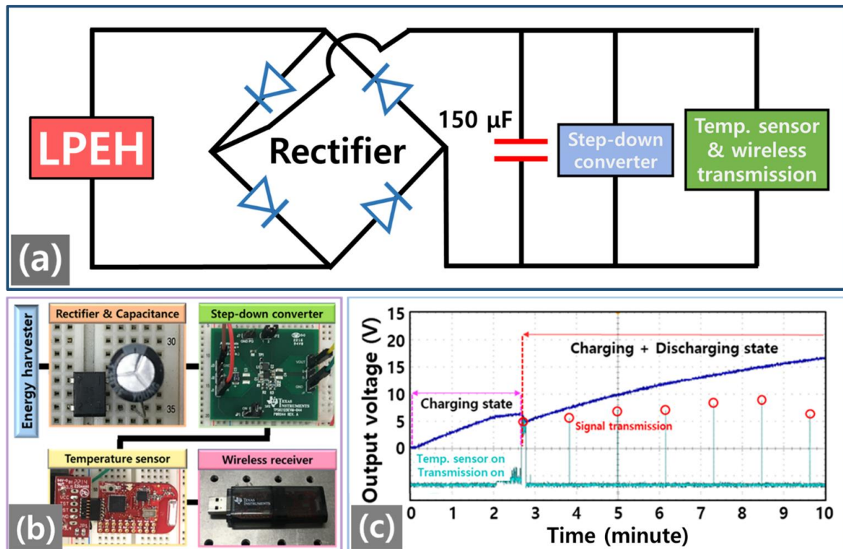
Fig. 4 (a) Circuit diagram of self-powered wireless temperature monitoring system powered with the LPEH in a magnetic field of 250 \mu\text{T} . (b) Photograph images of the self-powered wireless temperature monitoring system. (c) Characteristics of the self-charging voltage that drives the temperature sensor and RF transmission using a capacitor of 150 \mu\text{F} with the LPEH in a magnetic field of 250 \mu\text{T} .
