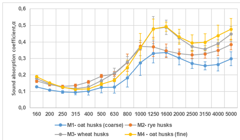
Figure 6. Results of the sound absorption coefficient of different MBC samples.
