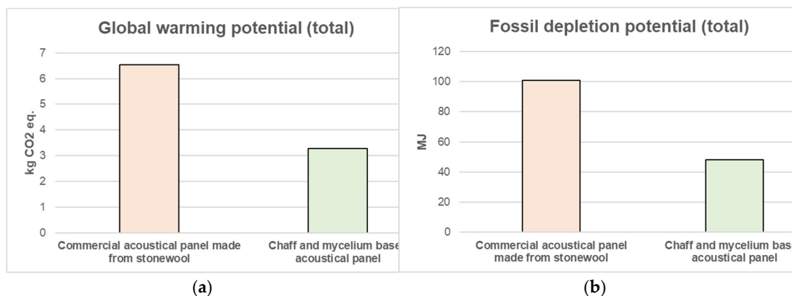
Figure 7. Global warming potential and fossil depletion potential results: (a) Global warming potential comparison between MBC acoustic insulation panel and stone wool panel; (b) Fossil depletion potential comparison between MBC acoustic insulation panel and stone wool panel.
