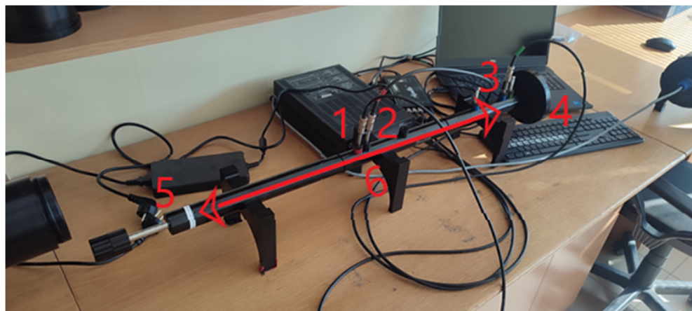
Figure 4. Impedance tube used during acoustic testing.
