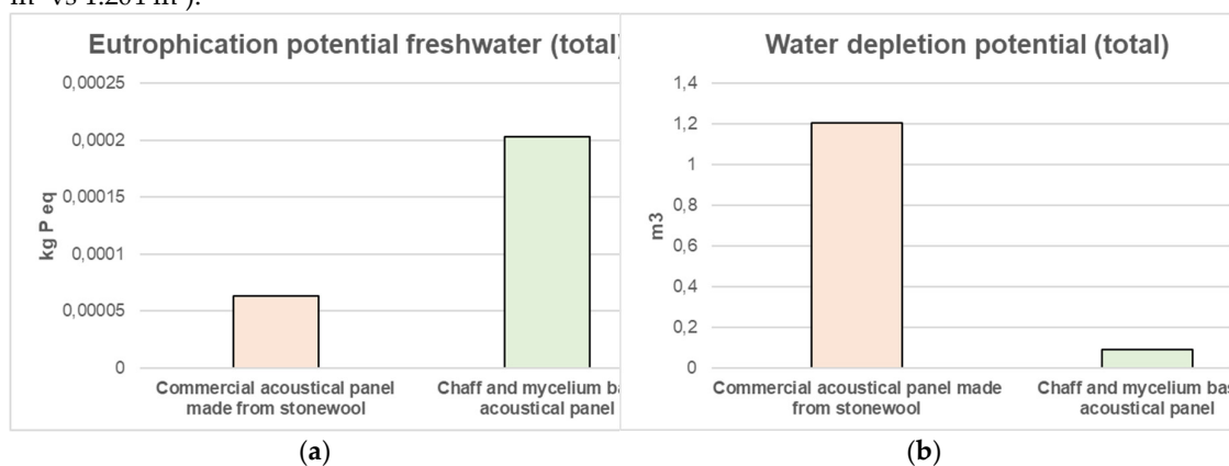
Figure 8. Eutrophication potential (freshwater) and water depletion potential results: (a) Eutrophication potential (freshwater) comparison between MBC acoustic insulation panel and stone wool panel; (b) Water depletion potential comparison between MBC acoustic insulation panel and stone wool panel.
