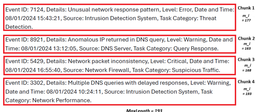
Figure 6. DFIR Context-Specific Chunking.
