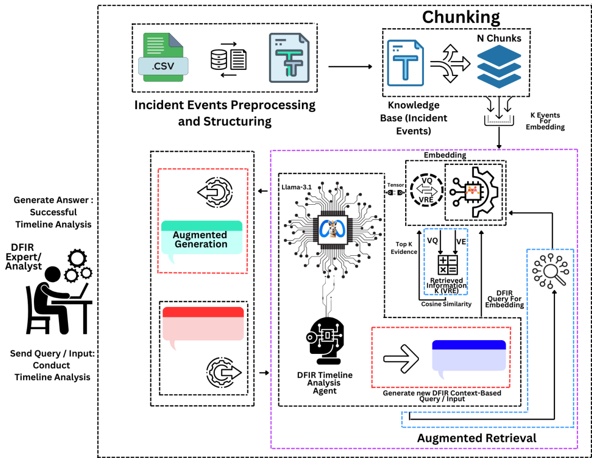
Figure 7. GenDFIR Framework Workflow.
