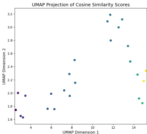
Figure 14. Unauthorised Access - Evidence (Top K=25)
