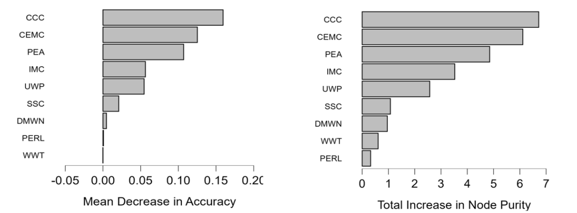
Figure 1. Mean Decrease in Accuracy and Total Increase in Node Purity.
