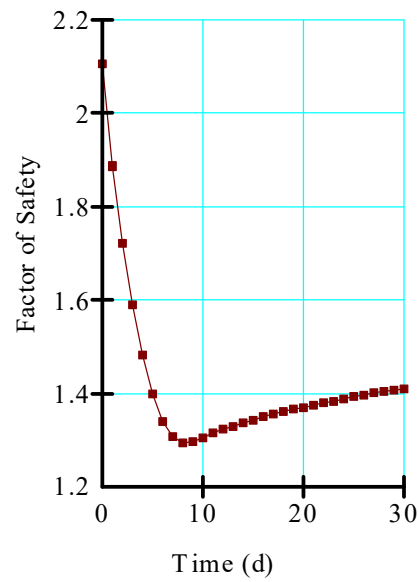
Figure 5. – Graph of the factor of safety values from 10 kN/m² cohesion material.
