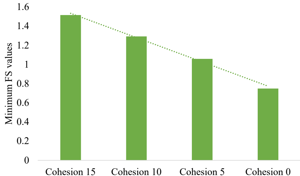
Figure 7. Summary of the minimum factor of safety values from the studied cohesion values.
