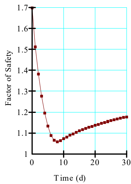
Figure 4. – Graph of the factor of safety values from 5 kN/m² cohesion material.
