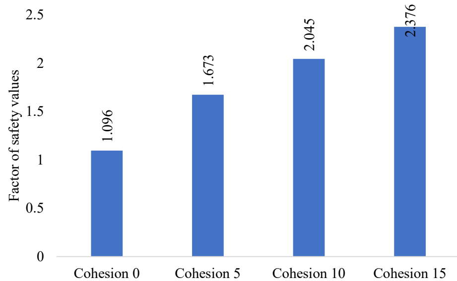
Figure 2. – Factor of safety values from long-term steady-state conditions.
