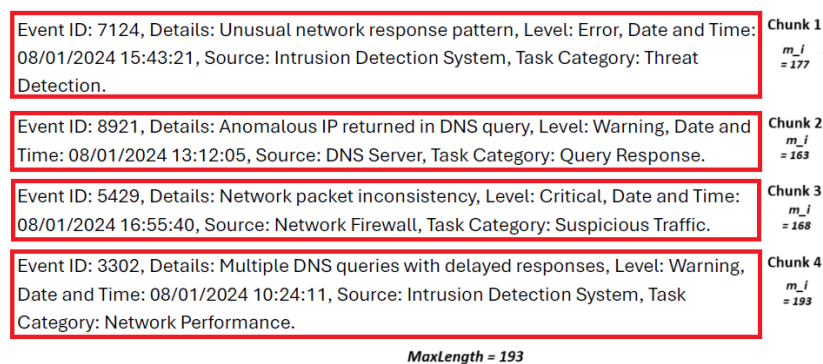
Figure 6. DFIR Context-Specific Chunking
