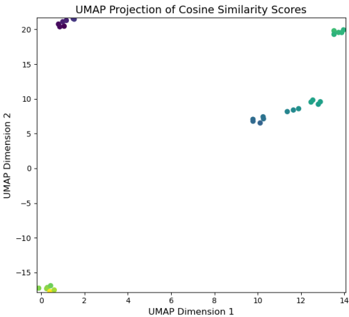
Figure 10. SYN Flood - Evidence (Top K=5)
