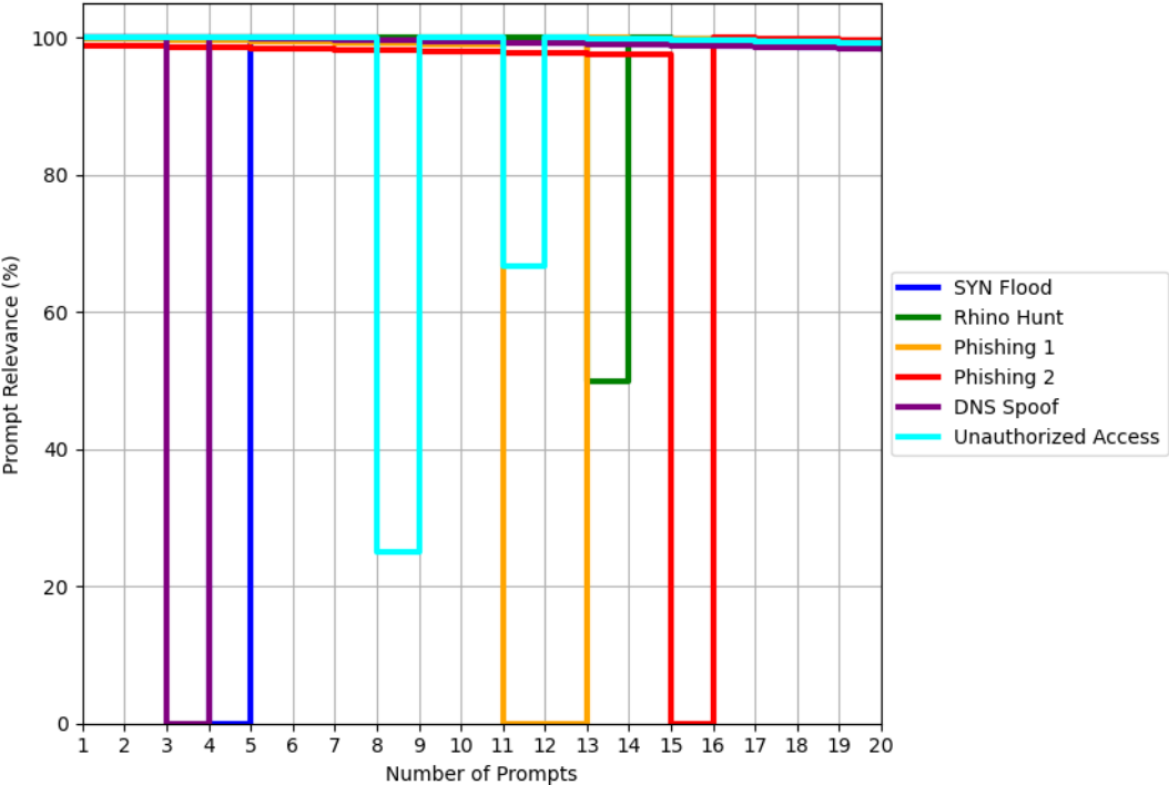
Figure 9. Prompts Relevance of GenDFIR Timeline Analysis reports for different Cyber Incident Scenarios.
