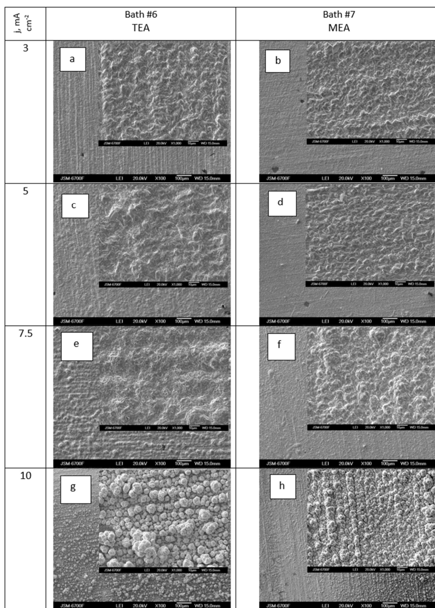
Figure 11. SEM images of samples obtained in dicyanoargentate-perrhenate electrolyte ( \text{KAg}(\text{CN})_2 - 0.11M; \text{KReO}_4 - 0.055M) with additions of 0.06 mol L -1 triethanolamine (a, c, e, g) and 0.165 mol L -1 monoethanolamine (b, d, f, h) at current density, mA cm -2 : 3 (a, b); 5 (c, d); 7.5 (e, f); 10 (g, h). Temperature 50°C.
