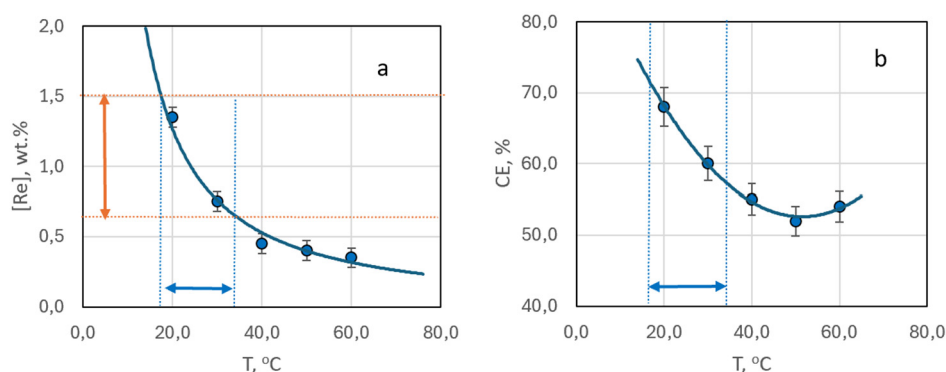
Figure 7. The mass fraction of rhenium in the deposit (a) and current efficiency (b) depending on the deposition temperature. The samples obtained from bath #2 at current density 3 \text{ mA cm}^{-2} without stirring.
