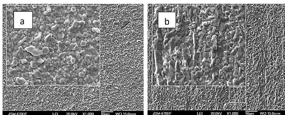
Figure 8. SEM images of samples obtained from baths with the [Ag^+]:[ReO_4^-] ratio: 10:1 (a), and 1:5 (b). Current density 10 \text{ mA cm}^{-2} , temperature 20^\circ\text{C} .
