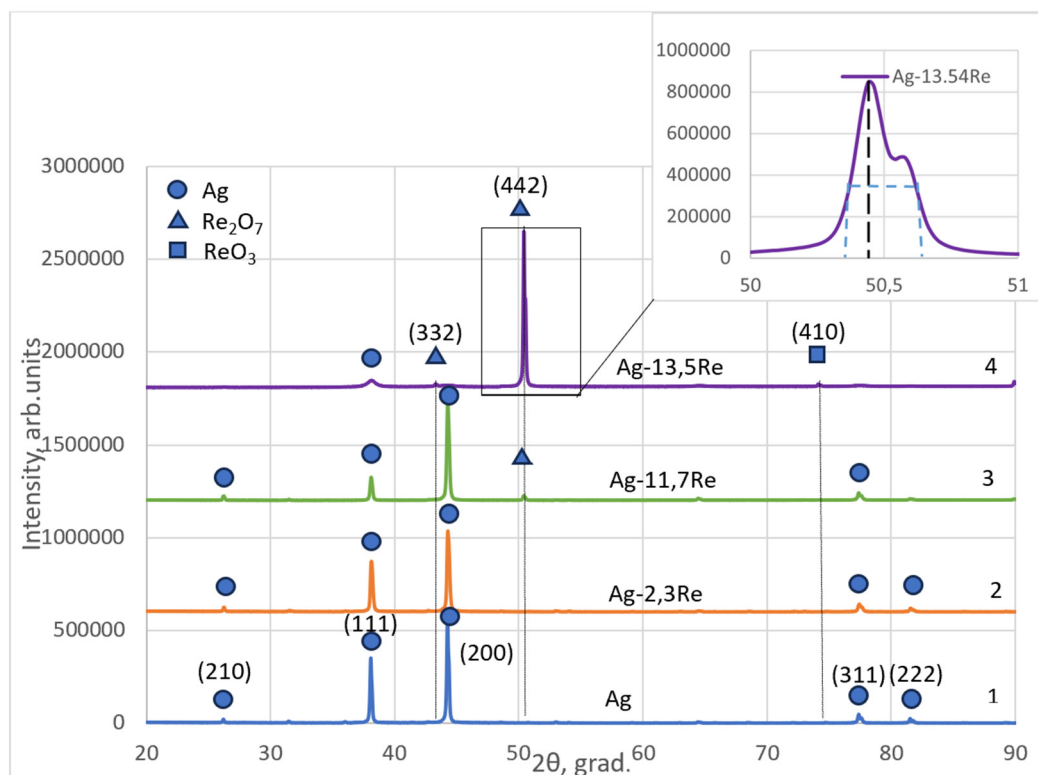
Figure 12. X-ray spectra electroplated silver (curve 1) and silver-rhenium coatings deposited from baths with different [Ag^+]:[ReO_4^-] ratio: 10:1 – 2; 1:1.5 – 3; 1:10 – 4.
