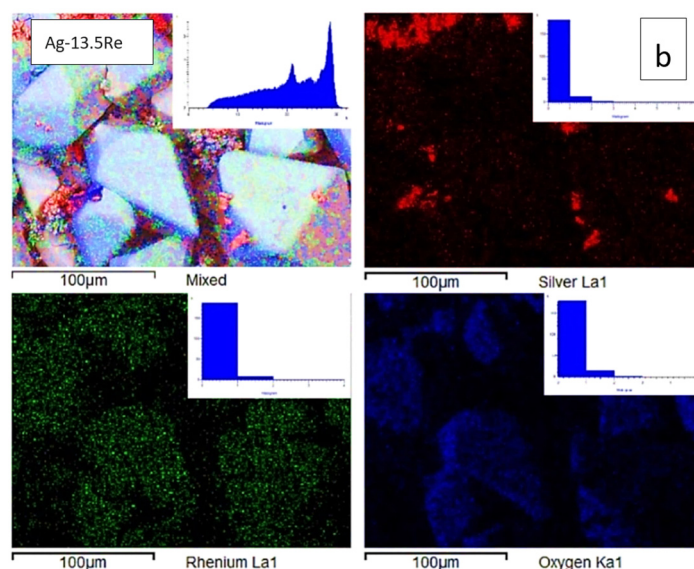
Figure 9. SEM images, corresponding elemental maps of Ag, Re and O of sintered samples Ag-2.3Re (a) and Ag-13.5Re (b).
