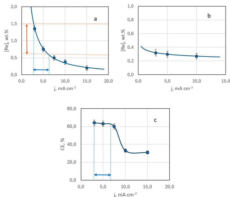
Figure 5. The mass fraction of rhenium in the deposit (a, b) and current efficiency (c) depending on the deposition current density. Electrolysis temperature, °C: 20 – a, c; 60 – b.
