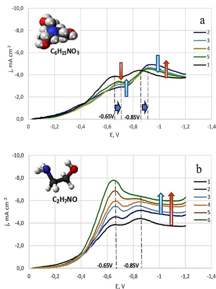
Figure 4. Potentiodynamic cathodic curves in dicyanoargentate-perrhenate silver electrolyte without surfactant (bath #5) - curve 1, and with the addition of triethanolamine (bath #6) (a), and monoethanolamine (bath #7) (b)
