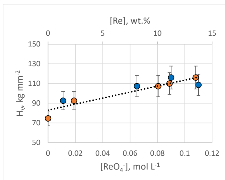
Figure 14. Dependence of the microhardness of Ag-Re coatings on the content of rhenium ions in the bath (blue dots) and the mass fraction of rhenium in the deposit (orange dots).
