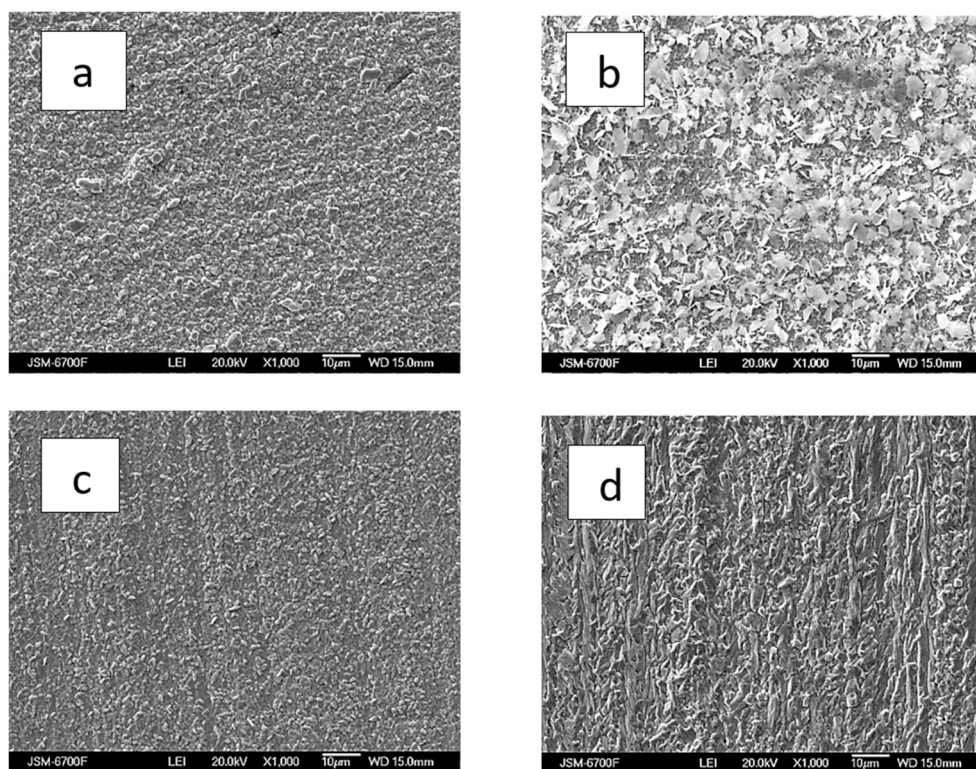
Figure 6. SEM images of samples obtained from bath #2 at current densities, \text{mA cm}^{-2} : 3 – a; 15 – b, c, d; and temperature, ^{\circ}\text{C} : 20 – a, c, 50 – b, 60 – c, d; without (a-c) and with stirring (d). The thickness of the coatings is 2–2.5 \mu\text{m} .
