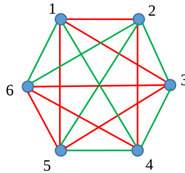
Figure 2. Bi-colored, complete, Ramsey graph generated by the vectors of momentum of the particles \vec{p}_i, i = (1 \dots 6) , and colored with red and green according to the Eqs. 3-4 is demonstrated. Vectors of momenta \vec{p}_i, i = (1 \dots 6) are the vertices of the graph.
