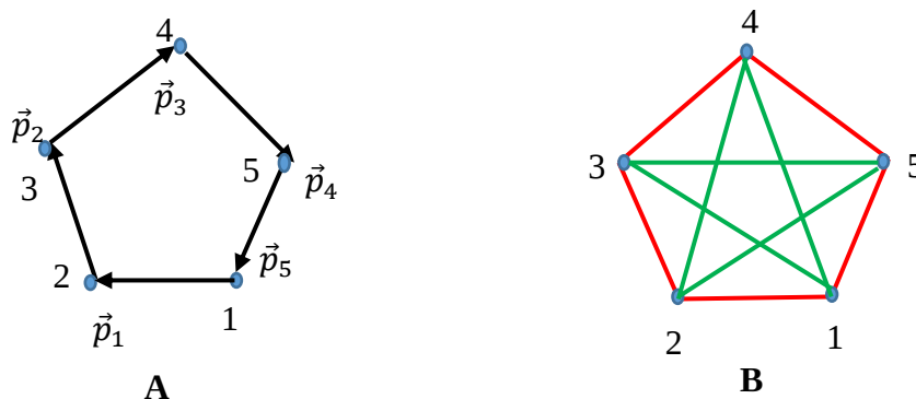
Figure 5. Ramsey complete bi-colored graph emerging from the system of five momenta vectors forming pentagon. A. \vec{p}_1 \dots \vec{p}_5 momenta vectors are depicted. B. Complete bi-colored graph emerging
