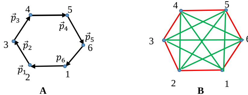
Figure 4. Ramsey complete bi-colored graph emerging from the system of six vectors of momenta, forming hexagon, is shown. A. \vec{p}_1 \dots \vec{p}_5 generating momenta vectors, forming a ring are depicted. |\vec{p}_i| = \text{const} takes place. B. Complete bi-colored graph emerging from the system of generating vectors \vec{p}_1 \dots \vec{p}_6 is shown. Eqs. 3-4 establish the green-red coloring of the graph. Triangles “135” and “246” are monochromatic/green.
