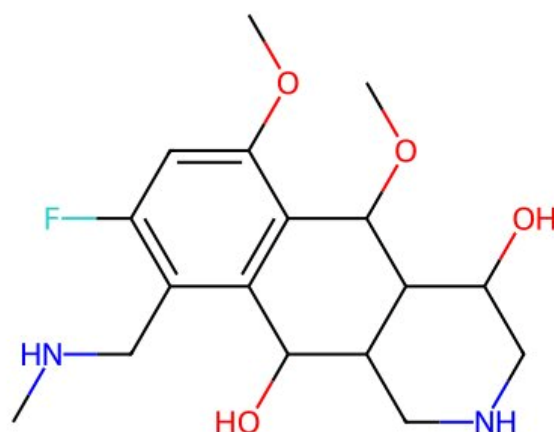
Figure 1. M6-12 generated via RDKit. C_{17}H_{25}FN_2O_4 , MW = 340.3950. SMILES: CNCc1c(F)cc(OC)c2c(OC)c3c(O)CNCC3c(O)c12 . Validated properties: LogP = 0.4847 (Crippen), TPSA = 82.98 Å 2 , HBD = 4, HBA = 6 (Lipinski), Fraction Csp3 = 0.6471, Rotatable bonds = 4.
