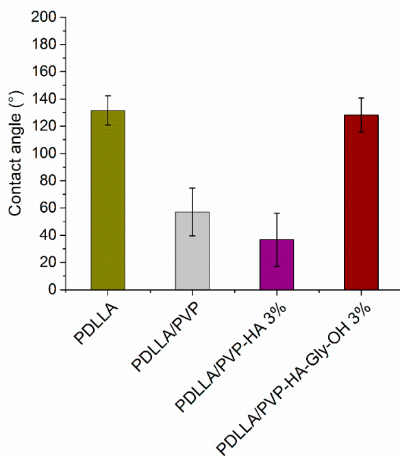
Figure 5. Mean contact angle values ( \pm standard deviation) for electrospun mats of PDLLA, PDLLA/PVP, PDLLA/PVP-HA 3%, and PDLLA/PVP-HA-Gly-OH 3%.
