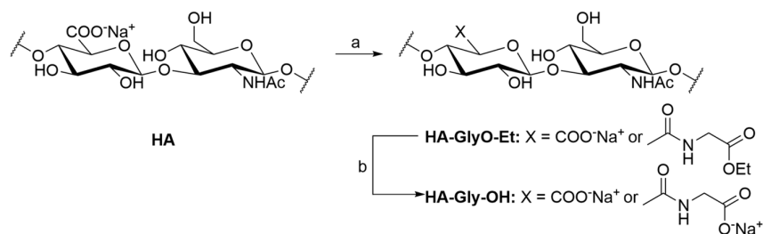
Scheme 1. Semi-synthesis of derivative HA-Gly. a: GlyOEt·HCl, EDC·HCl, s-NHs, MES, H 2 O, pH = 6, RT, overnight, yield = 77%, DS = 0.25; b: NaOH, H 2 O, pH = 12, RT, 6h, yield = 70%, DS = quantitative.
