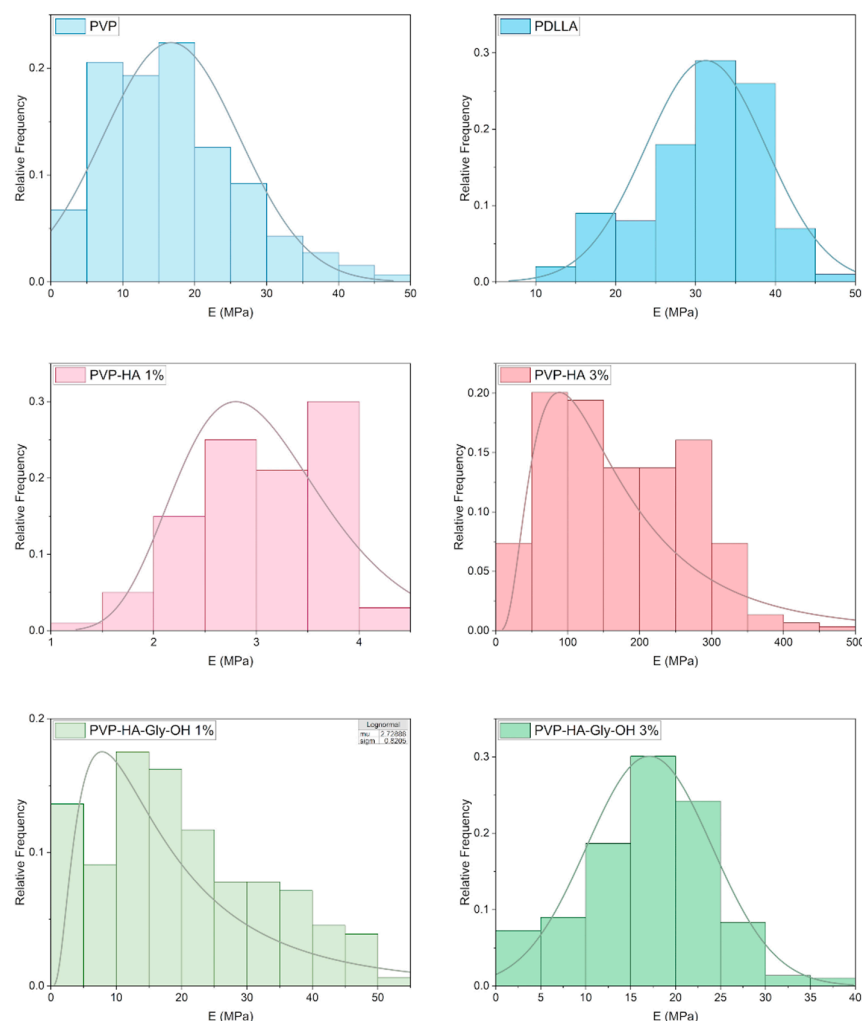
Figure 7. Histogram of electrospun scaffolds Young Modulus (E) distributions for neat PVP, neat PDLLA, PVP-HA 1%, PVP-HA 3% and PVP-HA-Gly-OH 1%, and PVP-HA-Gly-OH 3%. Every distribution is based on 300 acquisitions.
