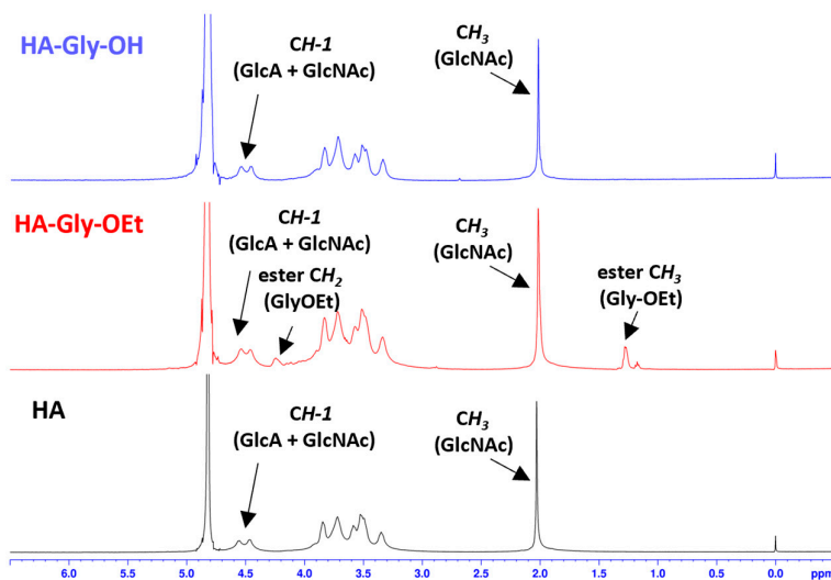
Figure 1. 1 H NMR spectra of HA (black), HA-Gly-OEt (red), and HA-Gly-OH (blue) (500 MHz, D 2 O, 25 °C).
