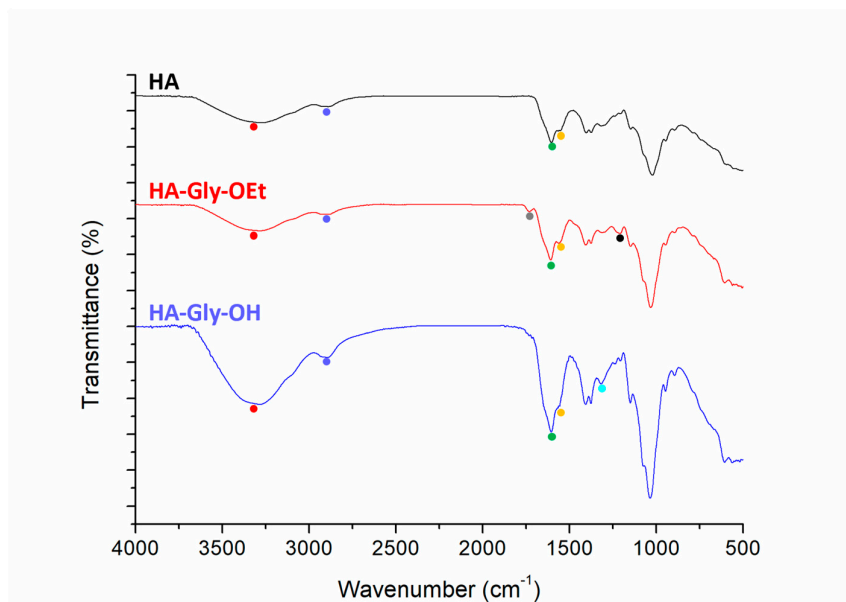
Figure 2. ATR FT-IR spectra of HA (black), HA-Gly-OEt (red), and HA-Gly-OH (blue). O-H and N-H stretching vibration band (red circle), C-H and C-H 2 stretching vibration (blue circle), ester C=O stretching vibration (grey circle), amide and carboxylate C=O stretching vibration (green circle), amide C-N and carboxylate C=O stretching vibration (orange circle), C-H 2 bending vibration (turquoise circle), ester C-O stretching vibration (black circle).
