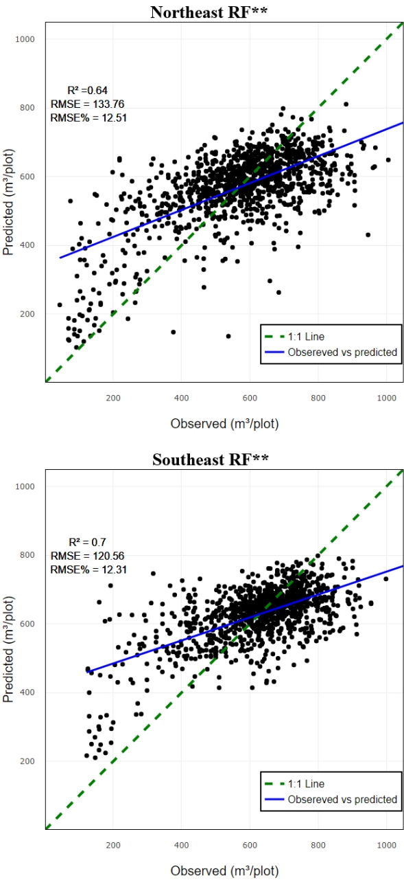
Figure 3. Scatter plot of observed vs. predicted GSV values for the validation plots using the best predictive model. The symbols * and ** represent the CO3 and CO4 combinations, respectively. Northwest RF, Southwest RF, Northeast RF, and Southeast RF denote the Random Forest-based models for the northwest, southwest, northeast, and southeast regions, respectively.
