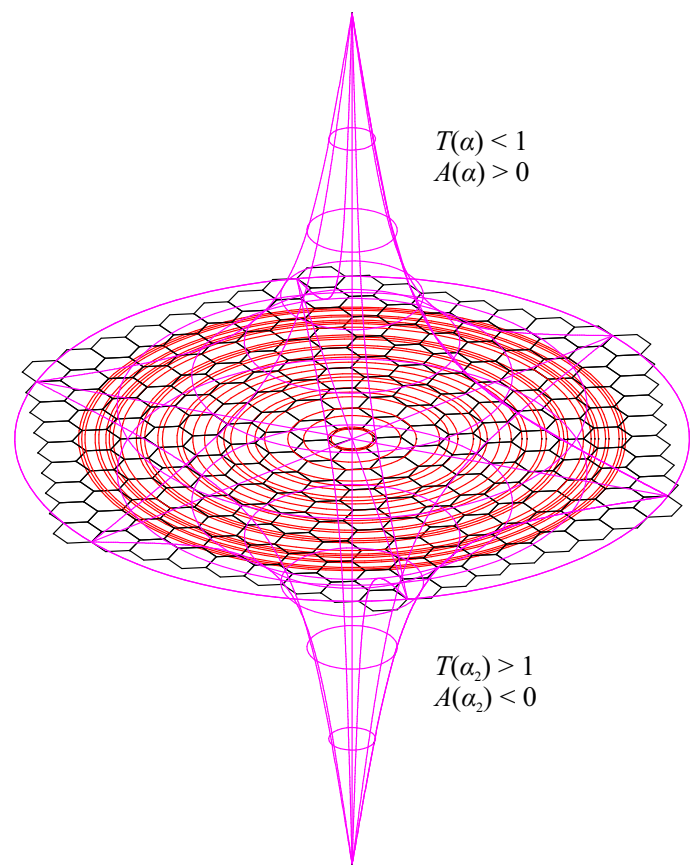
Figure 1. Illustration of the concepts of negative absorptance and excessive transmittance of EMR under normal incidence on MLG.
