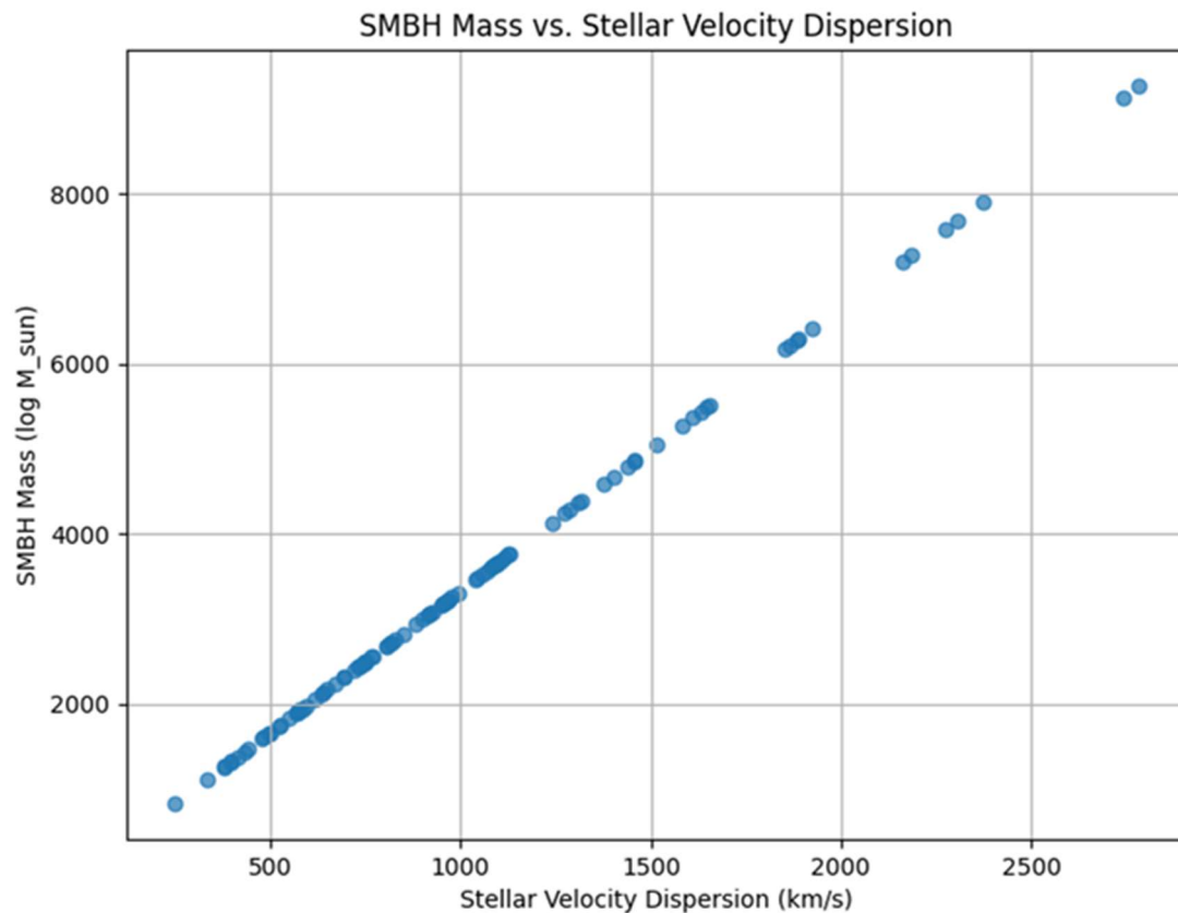
Figure 1. SMBH Mass vs. Stellar Velocity Dispersion This scatter plot illustrates the relationship between the mass of supermassive black holes (SMBHs) and the stellar velocity dispersion of their host galaxies. The positive correlation suggests that higher SMBH masses are typically found in galaxies with greater stellar velocity dispersions, reinforcing the M-sigma relation.
