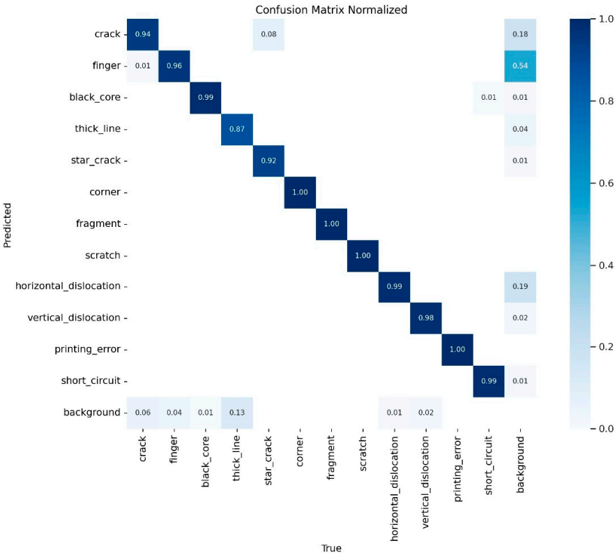
Figure 6. Normalized confusion matrix for the YOLOv10 model on the EL Solar Cells dataset. This matrix illustrates the model’s classification accuracy across different defect classes, with diagonal elements representing correct predictions and off-diagonal elements indicating misclassifications.
