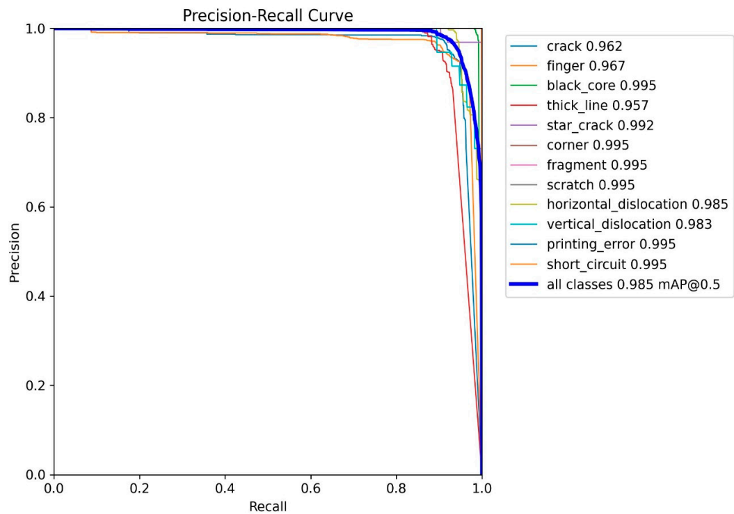
Figure 6. Precision-Recall Curve for the YOLOv10 model on the EL Solar Cells dataset. The curve illustrates the trade-off between precision and recall for each defect class, providing a comprehensive view of the model’s detection capabilities. The mean Average Precision (mAP@0.5) across all classes is 0.985, indicating the model’s high effectiveness in detecting a wide range of defects.”.
