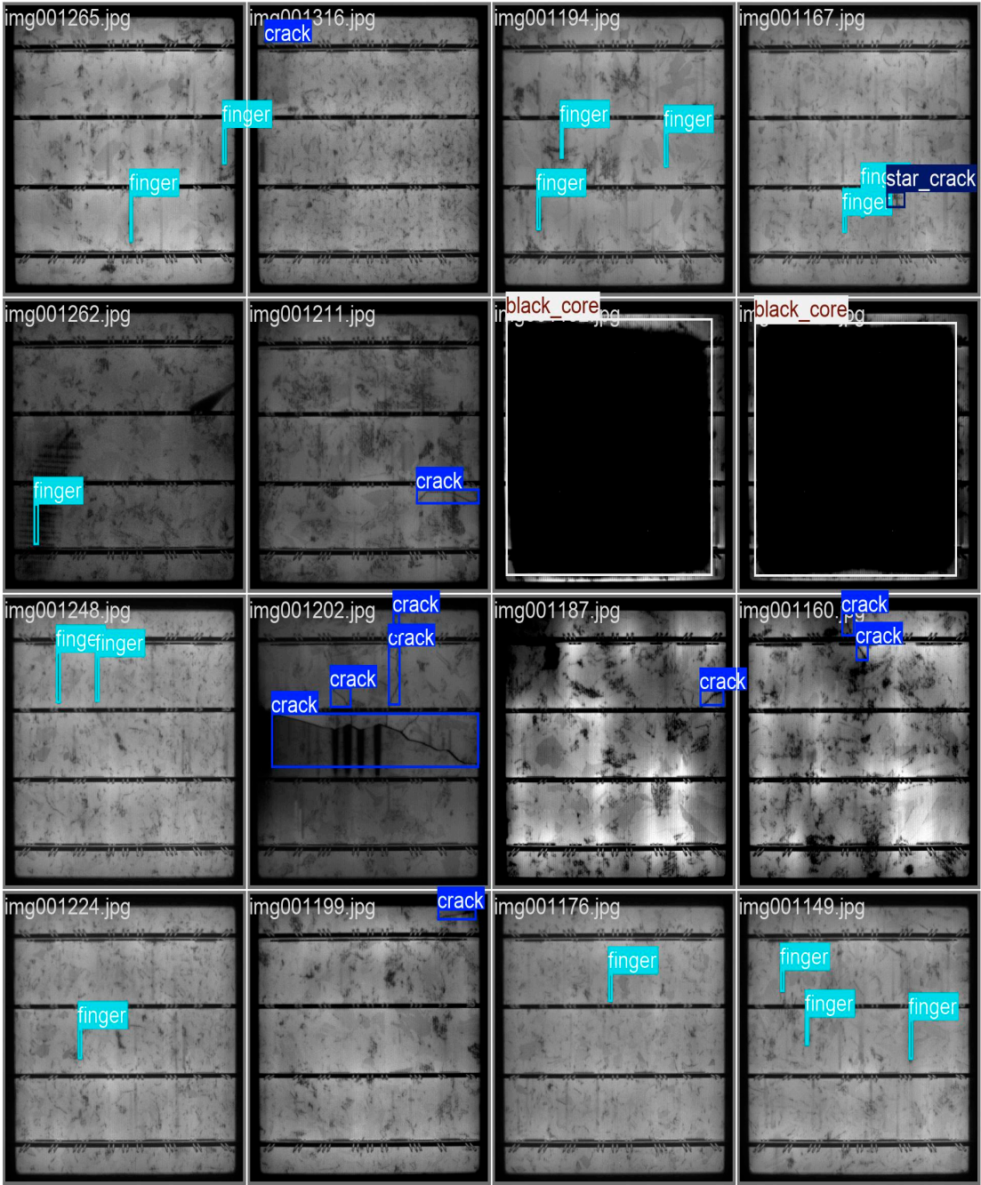
Figure 5. Detection results of the YOLOv10 model on the EL Solar Cells dataset. The figure shows various defect types, including cracks, finger interruptions, star cracks, and black core defects, with bounding boxes and labels indicating the detected defects. The images illustrate the model’s accuracy and capability in identifying and localizing multiple defect types.
