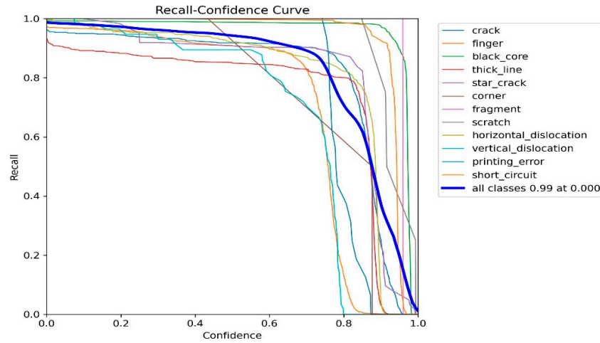
Figure 4. Recall-Confidence Curve for the YOLOv10 model across different defect classes in the EL Solar Cells dataset. The curve illustrates the relationship between recall and confidence threshold for each class, highlighting the model's detection performance and identifying areas where detection confidence varies among different defect types.
