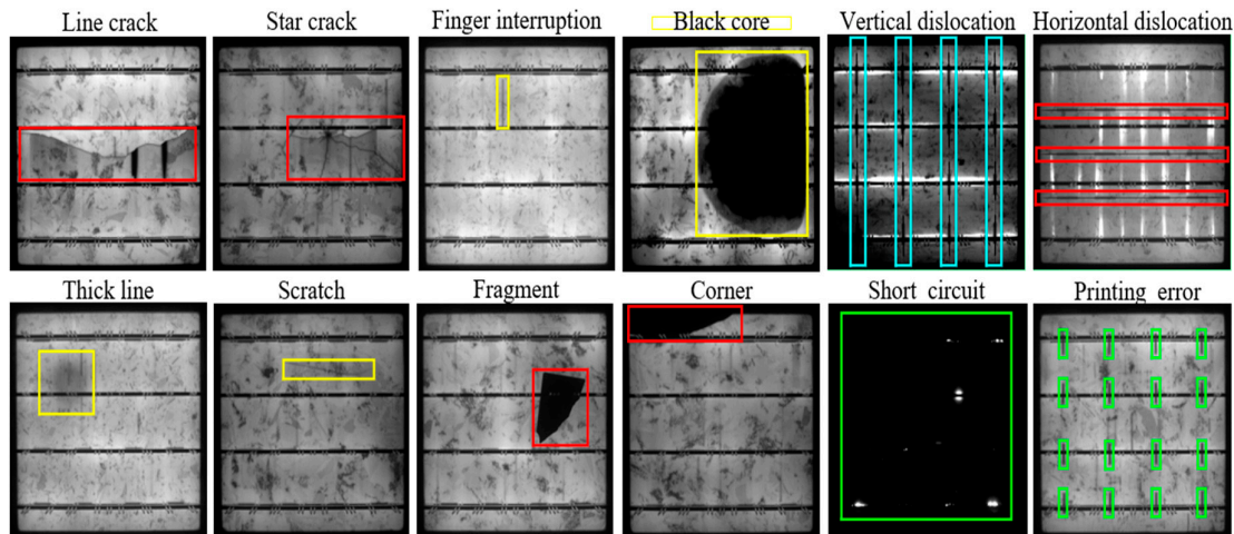
Figure 2. Examples of defect types in the EL Solar Cells dataset [27]. The dataset includes 12 classes of defects: Line crack, Star crack, Finger interruption, Black core, Vertical dislocation, Horizontal dislocation, Thick line, Scratch, Fragment, Corner, Short circuit, and Printing error. Each defect class is highlighted with colored bounding boxes for visual reference.
