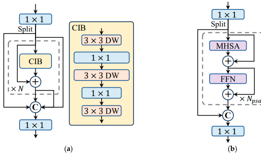
Figure 1. YOLOv10 model architecture: (a) The compact inverted block (CIB); (b) The partial self-attention module (PSA).
